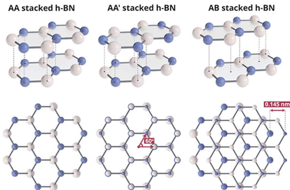
Fig. 1 Schematic diagram of the multi-type structure of h-BN. 7
