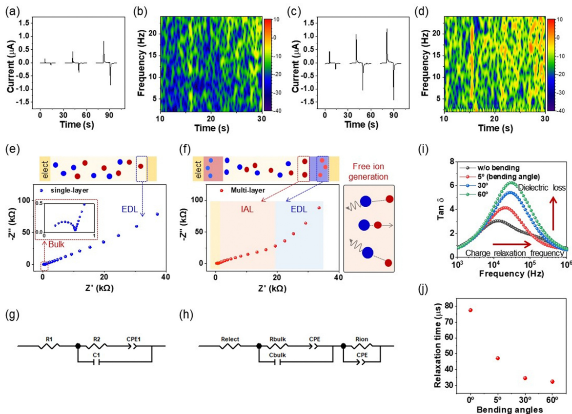
Fig. 4 Comparison of piezoionic performance between single-layer and multilayer sensors. (a) Current response of a single-layer sensor under bending deformations ( 5^\circ , 30^\circ , and 60^\circ ). (b) STFT spectral patterns of a single-layer sensor for the rough-surface scanning on a surface with gradient roughness. (c) Current response of a multilayer sensor under bending deformations ( 5^\circ , 30^\circ , and 60^\circ ) and (d) STFT spectral patterns of a single-layer sensor for the rough-surface scanning on a surface with gradient roughness. The color scale bar indicates the STFT intensity level. (e) Nyquist plot of the single-layer sensor, showing bulk film and EDL characteristics. (f) Schematic illustration of ion distribution in the single-layer configuration. (g) Equivalent circuit model for the single-layer sensor. (h) Modified equivalent circuit model for the multilayer sensor, incorporating ion accumulation effects. (i) Frequency-dependent \tan \delta curves showing charge relaxation frequency shifts with increasing bending deformation angles. (j) Relationship between the relaxation time and bending angle.
