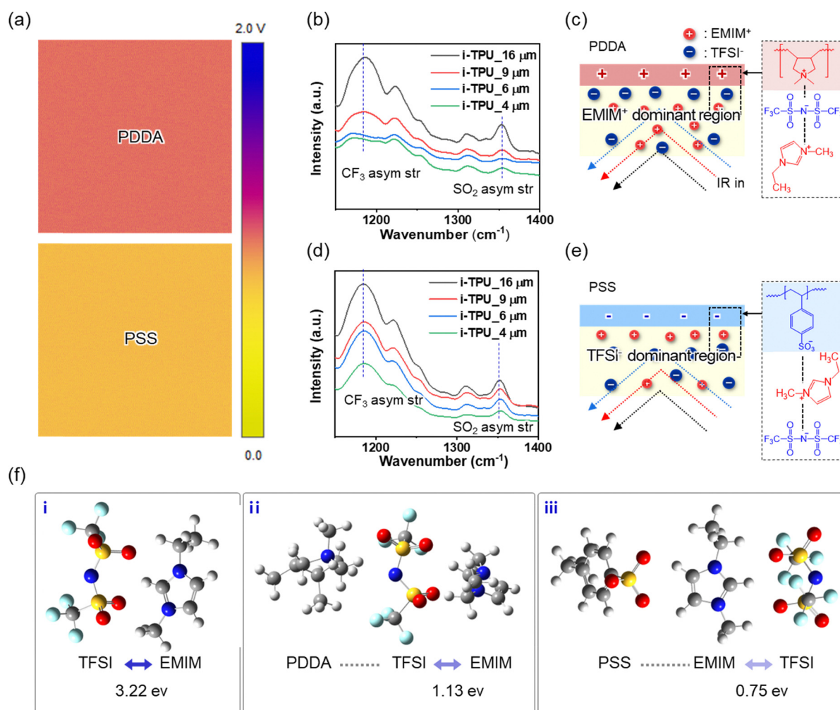
Fig. 2 Surface potential analysis and ion distribution characterization in the multilayer piezoelectric sensor. (a) Surface potential mapping of PDDA (top) and PSS (bottom) films, showing their distinct charge characteristics. (b) FT-IR spectra of active layers with varying thicknesses on the PDDA substrate, showing \text{TFSI}^- concentration variation with distance from the interface. (c) Schematic illustration of ion distribution near the PDDA interface, depicting \text{EMIM}^+ dominant regions formed by electrostatic interactions. (d) FT-IR spectra of active layers with varying thicknesses on the PSS substrate, indicating stable ion distribution. (e) Schematic representation of ion distribution near the PSS interface, showing \text{TFSI}^- dominant regions. (f) DFT-based binding energy calculations for (i) \text{TFSI}^- – \text{EMIM}^+ ion pair ( 3.22 \text{ eV} ), (ii) \text{PDDA} – \text{TFSI}^- – \text{EMIM}^+ interaction ( 1.13 \text{ eV} ), and (iii) \text{PSS} – \text{EMIM}^+ – \text{TFSI}^- interaction ( 0.75 \text{ eV} ), demonstrating reduced binding energy near charged layers.
