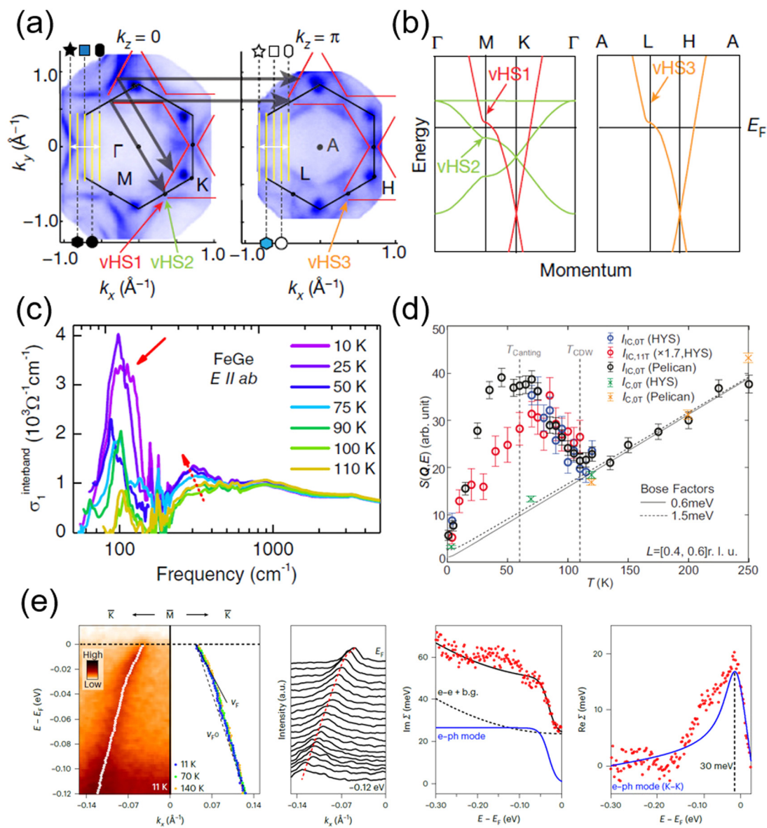
Fig. 11 (a) ARPES data showing the experimental observation of vHSs in FeGe. 49 (b) Schematic of the locations of vHSs in the electronic structure. 49 (c) Experimental observation of interband transfers below 100 K. 131 (d) Low energy spin structure and excitations as a function of temperature and field. 132 (e) Experimental observation of a dispersion kink and a bosonic mode at 30 meV. 130 (a) and (b) Are reproduced with permission from ref. 49. (c) Is reproduced with permission from ref. 131. (d) Is reproduced with permission from ref. 132. (e) Is reproduced with permission from ref. 130.
