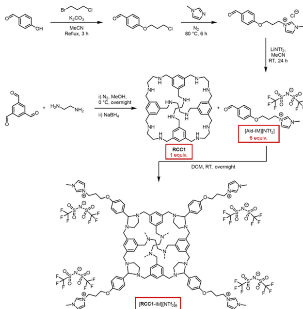
Fig. 1 Synthesis of ionic liquid functionalised aldehyde [\text{Ald-IM}][\text{NTf}_2] , reduced organic cage \text{RCC1} , and formation of an ionic liquid-functionalised cage [\text{RCC1-IM}][\text{NTf}_2]_6 – [\text{RCC1-IM}][\text{NTf}_2]_6 includes six aminated-tied ionic liquid functional groups but only four are shown for clarity, with the remaining two linking together the connected diamines via the dashed lines.
