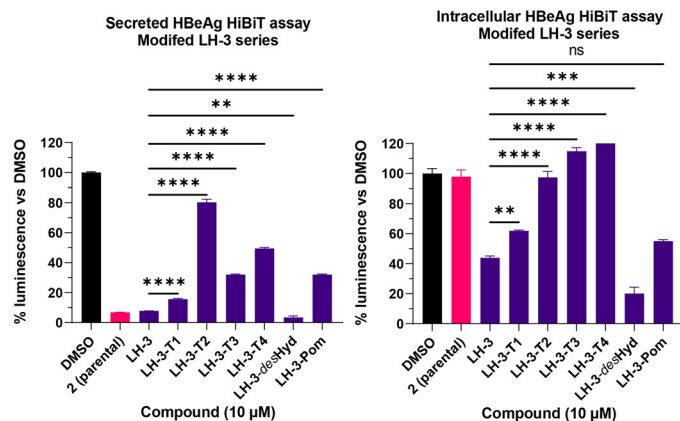
Fig. 4 A. A series of LH-3 analogues were prepared bearing truncated or altered E3L recruiting domains. B and C . HEK293T HiBiT-HBeAg-S cells were treated with LH-3 derivatives at 10 μM for 24 h then levels of secreted ( B ) and intracellular ( C ) HBeAg levels were assessed via HiBiT assay. Varying levels of activity against secreted HBeAg were observed, while only LH-3-T1, LH-3-desHyd and LH-3-Pom retained activity against intracellular HBeAg. **** represents P < 0.0001 , *** P \leq 0.001 , ** P \leq 0.01 , * P \leq 0.05 , ns = P > 0.05 as determined by one-way ANOVA. D . Consensus logP of LH-3 and derivatives were calculated using Swiss ADME, 44 and compared to activity against intracellular HBeAg. Relative activity is colour coded as high (green), moderate (yellow), or low (red).
