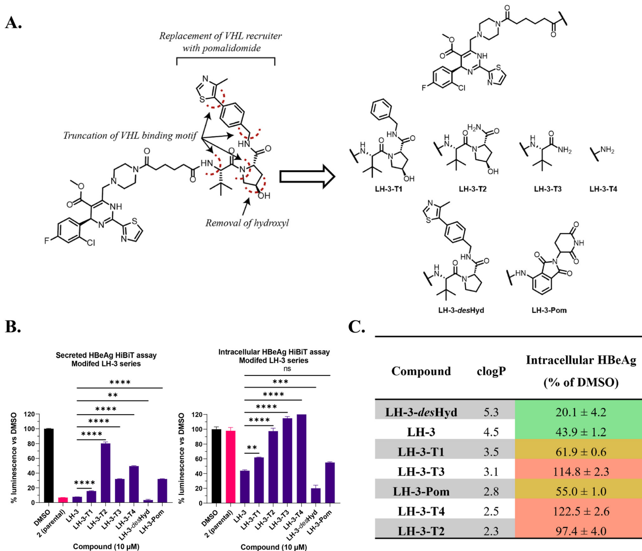
Fig. 4 A series of LH-3 analogues were prepared bearing truncated or altered E3L recruiting domains. B and C . HEK293T HiBiT-HBeAg-S cells were treated with LH-3 derivatives at 10 \mu M for 24 h then levels of secreted ( B ) and intracellular ( C ) HBeAg levels were assessed via HiBiT assay. Varying levels of activity against secreted HBeAg were observed, while only LH-3-T1, LH-3-desHyd and LH-3-Pom retained activity against intracellular HBeAg. **** represents P < 0.0001 , *** P \leq 0.001 , ** P \leq 0.01 , * P \leq 0.05 , ns = P > 0.05 as determined by one-way ANOVA. D . Consensus log P of LH-3 and derivatives were calculated using Swiss ADME, 44 and compared to activity against intracellular HBeAg. Relative activity is colour coded as high (green), moderate (yellow), or low (red).
