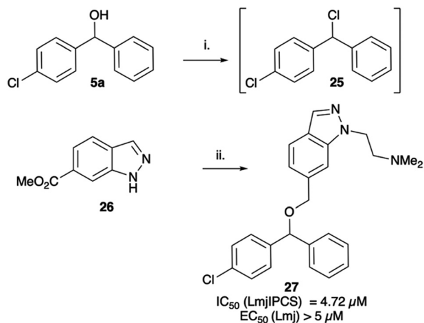
Scheme 3 Synthesis of indazole analogue 27 . i. MsCl , NEt_3 , DCM; ii. ClH-Me_2NCH_2CH_2Cl , K_2CO_3 , DMF, \Delta (54%), iii. LiAlH_4 , THF (100%); iv. NaH , DMF then add 25 (14%).
