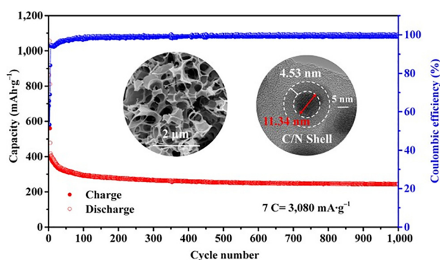
Fig. 26 Long-term cycling stability and structural integrity of the N-CQD-enhanced FeSb composite anode in PIBs. 206 Copyright 2022, Springer.
