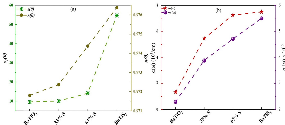
Fig. 10 Effect of sulfur doping on (a) static dielectric constant \epsilon_1(0) and refractive index n(0) and (b) absorption coefficient \alpha(\omega) and optical conductivity \sigma(\omega) .
