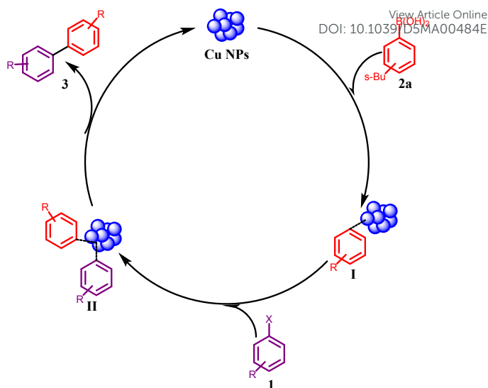
Figure 2: Plausible mechanism for copper nanoparticle catalysed Suzuki-Miyaura Coupling reaction.
