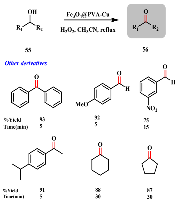
Scheme 26: Oxidation of alcohol to ketone catalysed by copper-based nanocomposite (Rahimi et al. )
