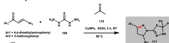
Scheme 49: Copper nanoparticles catalysed synthesis of 1,3,4-thiadiazole derivative compounds (Zeebaree et al. )
