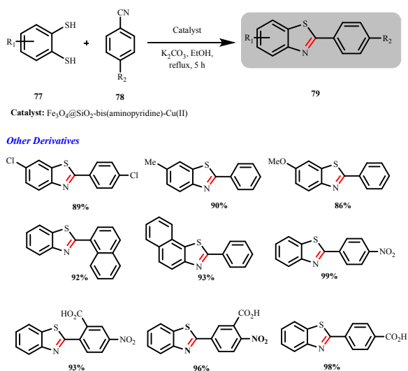
Scheme 37: Reaction between 2-aminobenzenethiol and benzonitrile catalyzed by \text{Fe}_3\text{O}_4@\text{SiO}_2\text{-bis(aminopyridine)-Cu(II)} nanocomposite. (Mahmood et al. )
