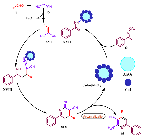
Figure 7: Plausible mechanism for synthesis of 2-aminonicotinonitrile using \text{CuI@Al}_2\text{O}_3 nanocatalyst
