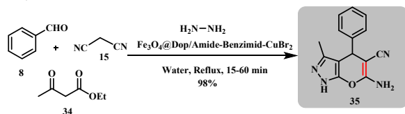
Scheme 14: \text{Fe}_3\text{O}_4@\text{Dop}/\text{amide-benzimid-CuBr}_2 catalysed synthesis of 6-amino-3-methyl-4-phenyl-1,4-dihydropyrano[2,3-c]pyrazole-5-carbonitrile (Li et al. )
