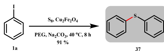
Scheme 20: \text{Cu}_2\text{Fe}_2\text{O}_4 catalysed synthesis of diphenylsulfane (Ichie et al. )
