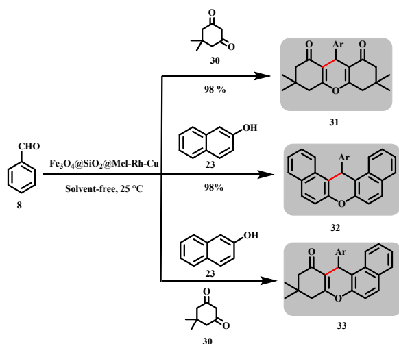
Scheme 13: \text{Fe}_3\text{O}_4@\text{SiO}_2@\text{NTMPThio-Cu} catalysed synthesis of Xanthenes. (Peiman et al. )
