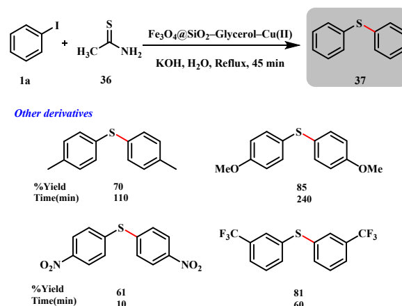
Scheme 15: \text{Fe}_3\text{O}_4@\text{SiO}_2\text{-Glycerol-Cu(II)} catalysed synthesis of sulfides (Ashraf et al. )
