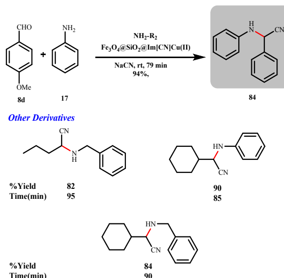
Scheme 39: Catalytic synthesis of \alpha -aminonitriles derivatives using \text{Fe}_3\text{O}_4@\text{SiO}_2@\text{Im}[\text{CN}]\text{Cu(II)} nanoparticles (Kazemnejadi et al. )
