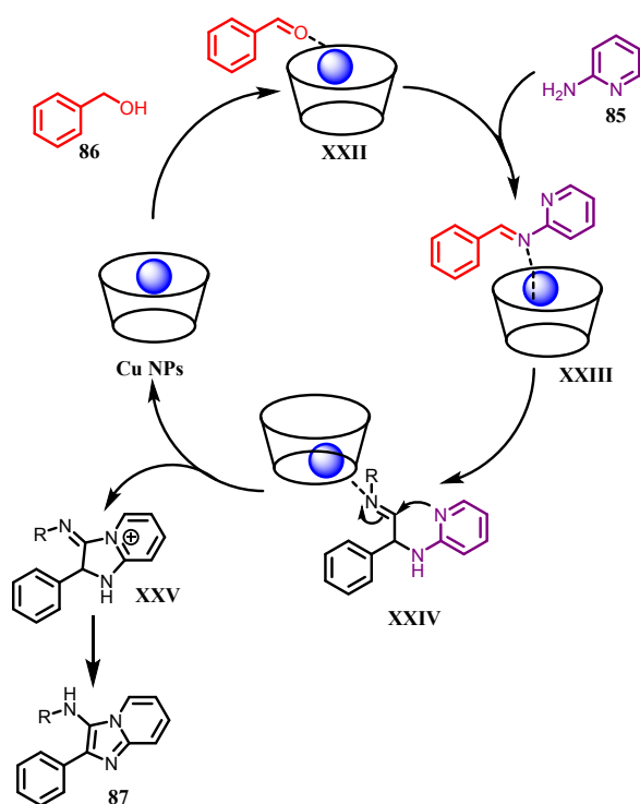
Figure 9: Plausible mechanism for synthesis of N -(alkyl)-2-phenylimidazo[1,2- a ]pyridin-3-amine derivatives using Cu@β-CD@MGO nanoparticles.
