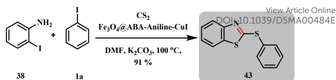
Scheme 19: \text{Fe}_3\text{O}_4@\text{ABA-Aniline-CuI} catalysed synthesis of 2-(phenylthio)benzo[d]thiazole (Sun et al. )
