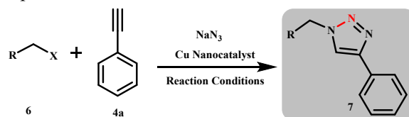
Scheme 3: General Click reaction
