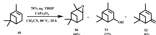
Scheme 23: Oxidation of pinene catalysed by copper ferrite nanoparticles (Mdletshe et al. )
