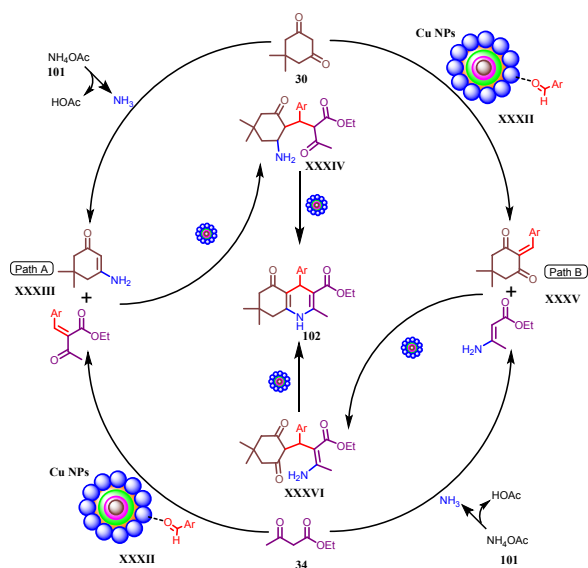
Figure 11: Plausible mechanism for synthesis of Hexahydroquinoline derivatives using \text{Fe}_3\text{O}_4@\text{SiO}_2@\text{Si}(\text{CH}_2)@\text{HMAT}@\text{Cu} nanocomposite.
