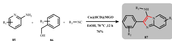
Scheme 40: Catalytic synthesis of N -(alkyl)-2-phenylimidazo[1,2- a ]pyridin-3-amine derivatives using Cu@β-CD@MGO nanoparticles (Bahadorikhalili et al. )
