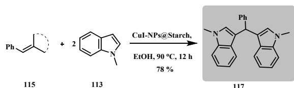
Scheme 51: Copper nanoparticles catalysed synthesis of bisindolylmethane (Suresh et al. )
