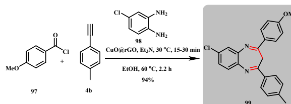
Scheme 44: Catalytic synthesis of 1,5-benzodiazepines derivatives using \text{CuO}@r\text{GO} nanocomposite. (Sarkar et al. )
