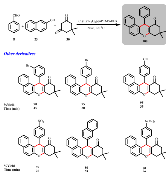
Scheme 45: Catalytic synthesis of heterocyclic derivatives using Cu(II)/ \text{Fe}_3\text{O}_4@\text{APTMS-DFX} nanocomposite (Sonei et al. )
