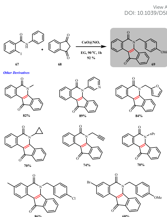
Scheme 33: \text{CuO@NiO} catalysed synthesis of indenoisoquinoline (Rawat et al. )
