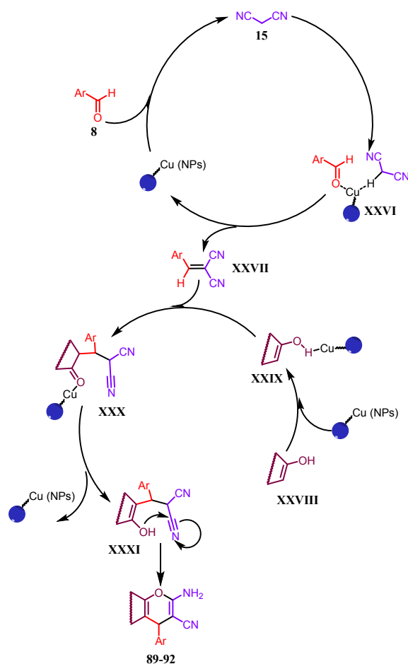
Figure 10: Plausible mechanism for synthesis of 2-amino-4H chromene derivatives using \text{Fe}_3\text{O}_4@\text{SiO}_2 -imine/phenoxy-Cu(II) nanoparticles (Ebrahimi et al. )
