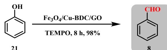
Scheme 25: Oxidation of phenol to benzaldehyde catalysed by \text{Fe}_3\text{O}_4\text{/Cu-BDC/GO} catalyst (Alamgholiloo et al. )
