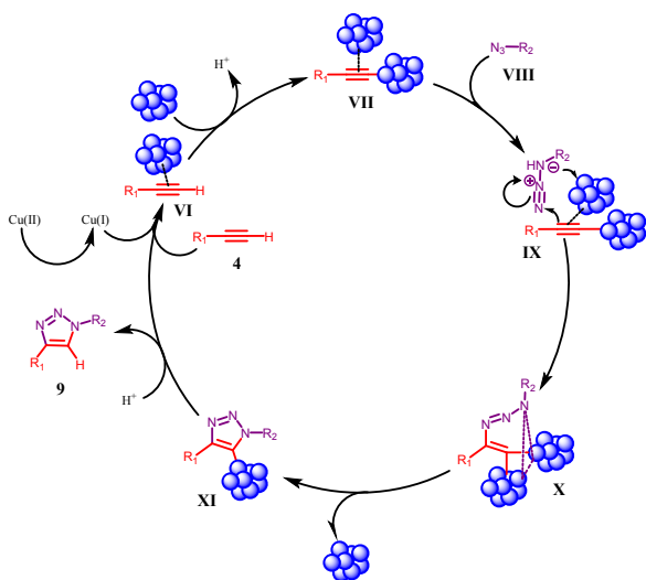
Figure 4: Plausible mechanism for copper nanoparticle catalyzed Click reaction.
