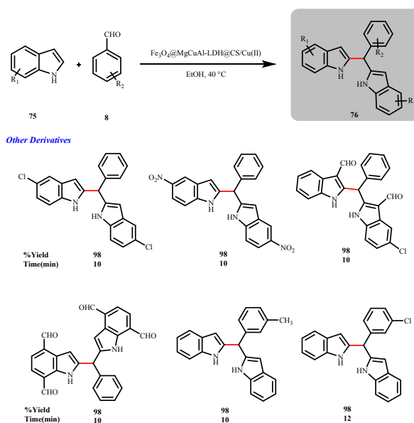
Scheme 36: Bis(indolyl)methanes synthesis in the presence of Fe 3 O 4 @MgCuAl-LDH@CS/Cu(II) (Rashtiani et al. )
