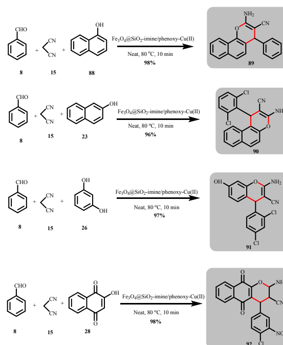
Scheme 41: Catalytic synthesis of 2-amino-4 H chromene derivatives using Fe 3 O 4 @SiO 2 -imine/phenoxy-Cu(II) nanoparticles (Ebrahimiasl et al. )
