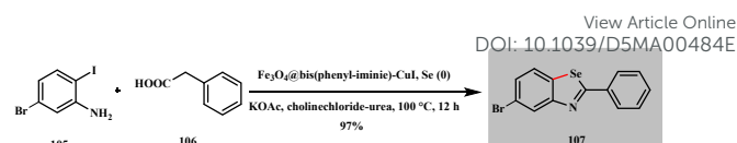
Scheme 48: \text{Fe}_3\text{O}_4@\text{bis}(\text{phenyl-imine})\text{-CuI} catalysed synthesis of 2-phenylbenzo[d][1,3]selenazole (Hu et al. )
