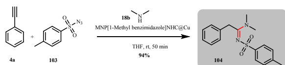
Scheme 47: Synthesis of N -sulfonyl amidine derivatives in presence of catalyst \text{MNP}[1\text{-Methyl benzimidazole}]\text{NHC}@\text{Cu} . (Pawar et al. )
