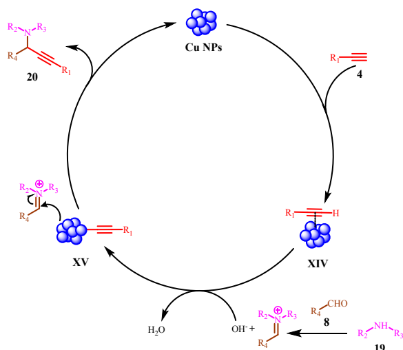
Figure 6: Plausible mechanism for copper nanoparticle catalysed A3 Coupling reaction.
