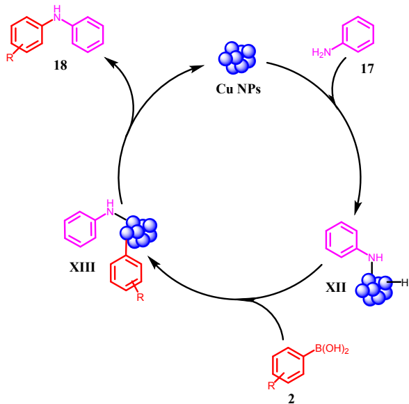
Figure 5: Plausible mechanism for copper nanoparticle catalysed Chan-Lam Coupling reaction.
