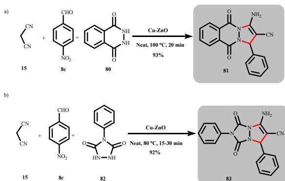
Scheme 38: Catalytic synthesis of heterocyclic derivatives using Cu-ZnO nanoparticles (Maleki et al. )
