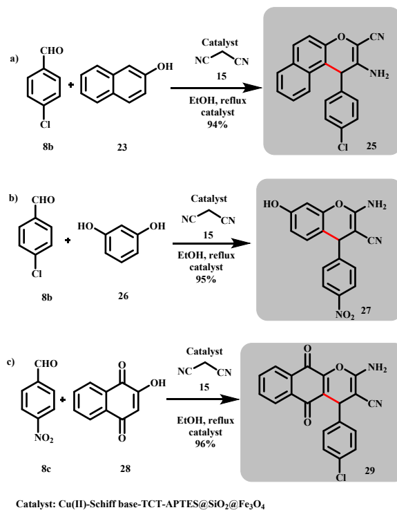
Scheme 12: Cu(II)-Schiff base-TCT-APTES@SiO 2 @Fe 3 O 4 catalysed synthesis of Chromene derivatives. (Kalantar et al. )
