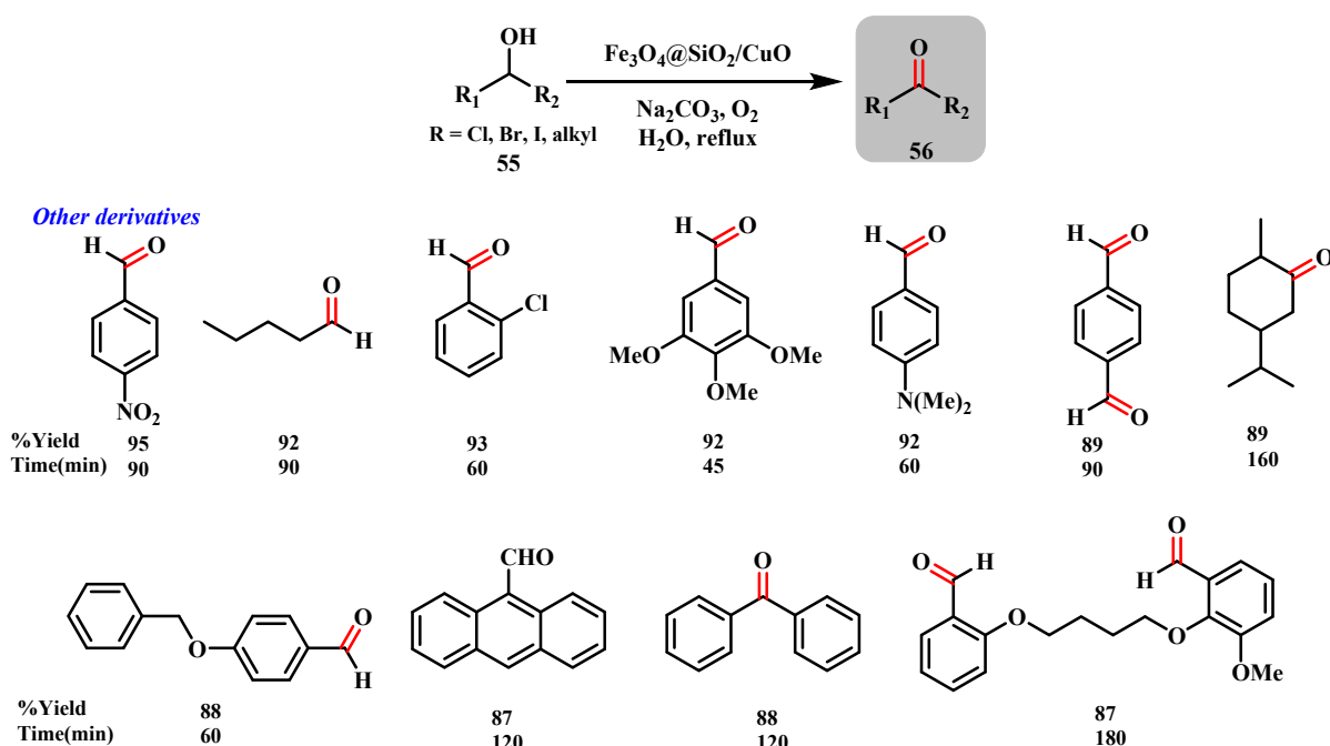
Scheme 26: Oxidation of alcohol to ketone catalysed by copper-based nanocomposite (Rahimi et al. )
