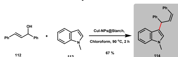
Scheme 50: Copper nanoparticles catalysed 3-allylation of indoles (Mallick et al. )
