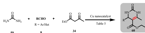
Scheme 29: Synthesis of DHPMs using copper based nanocatalyst
