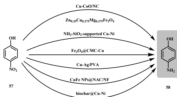
Scheme 28: Various copper-catalysts used in reduction reaction
