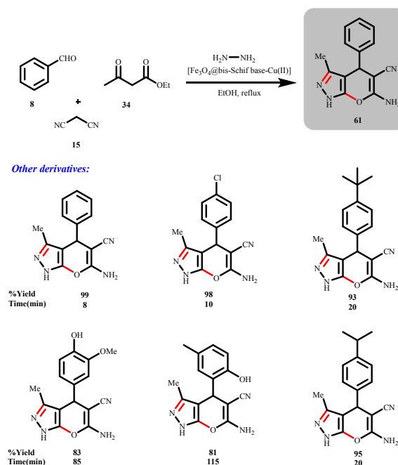
Scheme 30: Synthesis of pyrano[2,3- c ]pyrazoles using copper-based nanocatalyst (Ali et al. )
