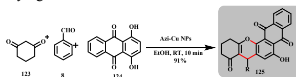
Scheme 54: Azi-Cu NPscatalysed one-pot synthesis of xanthene. (Selvaraj et al. )
