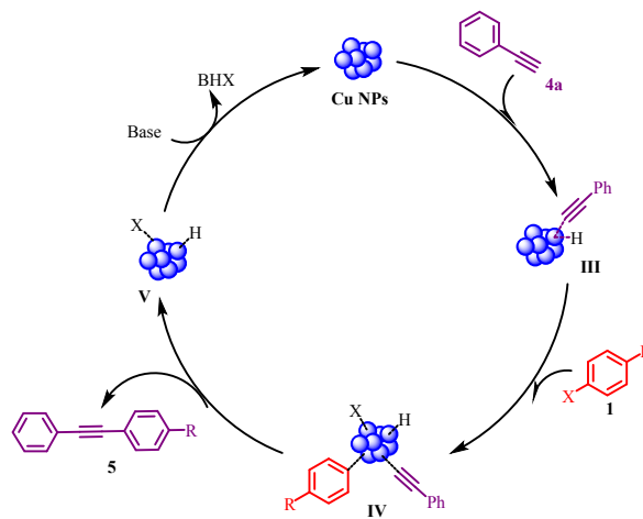
Figure 3: Plausible mechanism for copper nanoparticle catalysed Sonogashira Coupling reaction.
