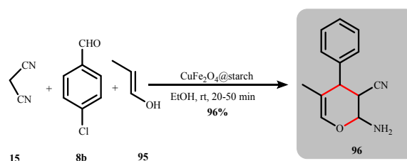
Scheme 43: Catalytic synthesis of 4 H -pyran derivatives using \text{CuFe}_2\text{O}_4@\text{starch} nanoparticles (Kamalzare et al. )
