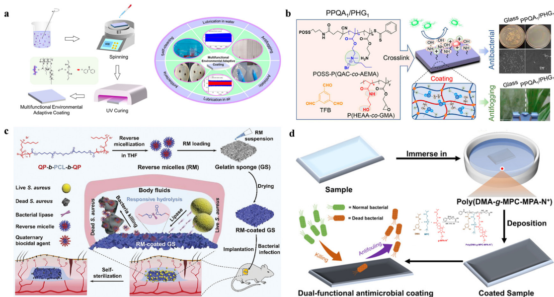
Fig. 21 (a) Preparation process of amphiphilic multifunctional environmental adaptive coating; reproduced with permission from ref. 174, copyright 2022, American Chemical Society. (b) Synthesis of POSS-P(QAC-co-AEMA) and P(HEAA-co-GMA) copolymers for antibacterial and antifogging coatings; reproduced with permission from ref. 175, copyright 2020, American Chemical Society. (c) Schematic illustration for the fabrication of RM-coated GS and the mechanism of bioswitchable self-sterilization in bacterial infection site; reproduced with permission from ref. 80, copyright 2021, Wiley. (d) Preparation process of poly(DMA-g-MPC-MPA-N + ) and dual-functional antimicrobial coating; reproduced with permission from ref. 176, copyright 2022, Elsevier.
