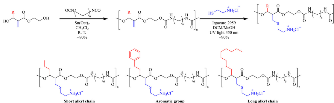
Fig. 6 Synthesis of antimicrobial surfactant-like poly(ester polyurethane)s with different hydrophobic pendant groups ( PSA , PA , and PLA ) and cationic groups distributed uniformly along the polymer chain. Redrawn from ref. 122.
