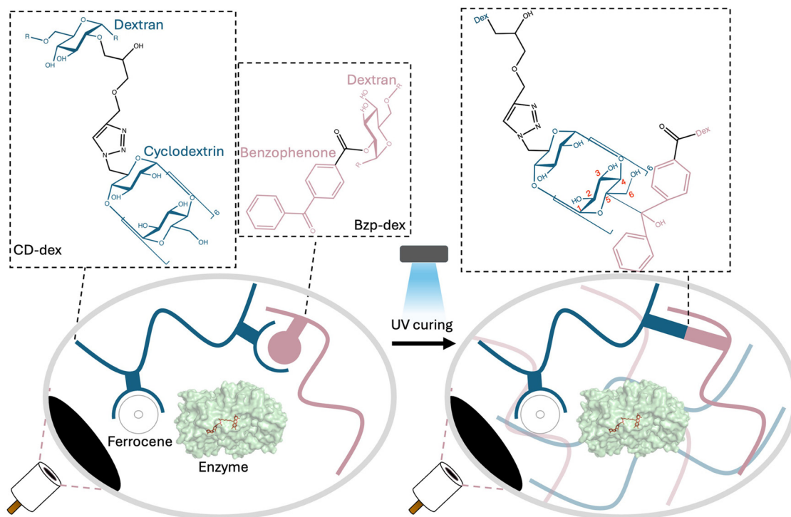
Scheme 1 Schematic drawing of the process of immobilizing and entrapping ferrocene and enzyme on an electrode surface within a UV cured hydrogel matrix. Note: there are likely several reaction routes between CD and Bzp, and Bzp may also bind to dex and/or the enzyme. However, due to the high tendency for Bzp to form inclusion complexes with CD and the stabilization effect of the hydrophobic cavity towards the Bzp ketyl radical, the former interaction is more favored. Here is a simplified illustration only showing the binding to the C5 position.
