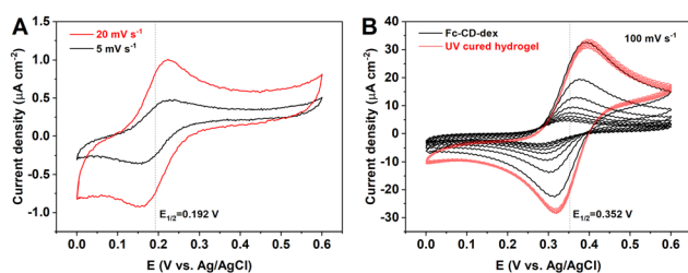
Fig. 1 Cyclic voltammograms (CVs) of (A) a bare GCE in 0.1 M pH 7 PBS containing free Fc with a saturated concentration and (B) modified GCEs with Fc-CD-dex and the UV cured hydrogel.
