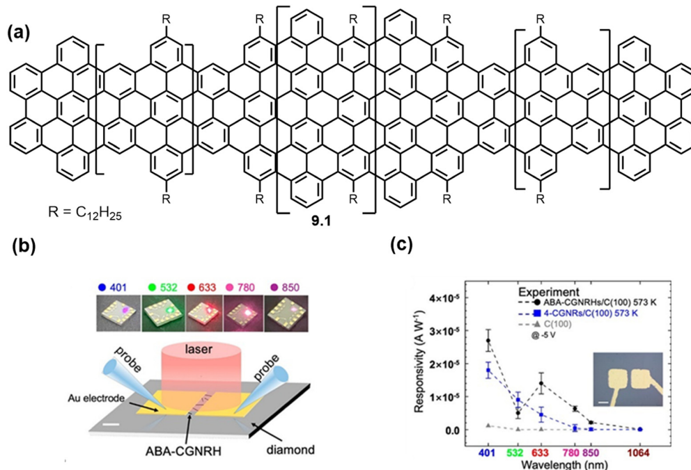
Fig. 11 (a) GNR heterostructures (9.1) synthesized for use in molecular diodes (b) Schematic I - V measurement of GNR-based device (100) (c) Average photoresponsivity of six GNR-based devices on diamond at 573 K and -5 V under vacuum conditions. 71 Reproduced from ref. 71 with permission from [ACS], copyright [2023].
