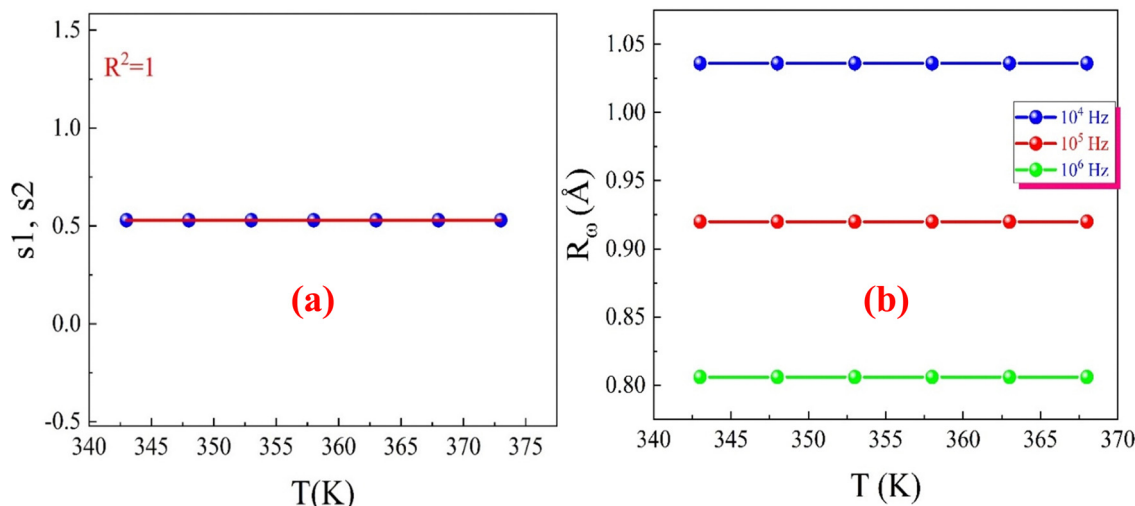
Fig. 16 (a) Temperature variation of the exponents “s”. (b) Thermal variation of the tunnelling distance R_0 , as a function of the frequency of the applied electric field for the eco-friendly synthesized CFO nanoparticles within the temperature range of 343–373 K.
