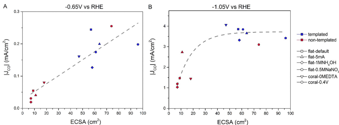
Fig. 6 Partial current densities to CO for both the template-based porous (blue) and non-templated equivalent (red) samples (n)t-flat-5mA, (n)t-flat-1MNH 4 OH, (n)t-flat-0.5MNaNO 3 , (n)t-coral-0MEDTA and (n)t-coral-0.4V at (A) -0.65 V vs. RHE and (B) -1.05 V vs. RHE plotted versus the ECSA. A dashed gray line is provided as a guide for the eye.
