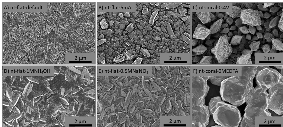
Fig. 3 SEM images of non-templated Ag electrodes prepared via Ag electrodeposition with different synthesis conditions: (A) default ( -0.1 V vs. Ag/AgCl, 0.05 M AgNO 3 , 1 M NaNO 3 , 0.01 M EDTA, 0.5 M NH 4 OH); (B) -5 mA; (C) -0.4 V; (D) 1 M NH 4 OH; (E) 0.5 M NaNO 3 ; (F) 0 M EDTA.
