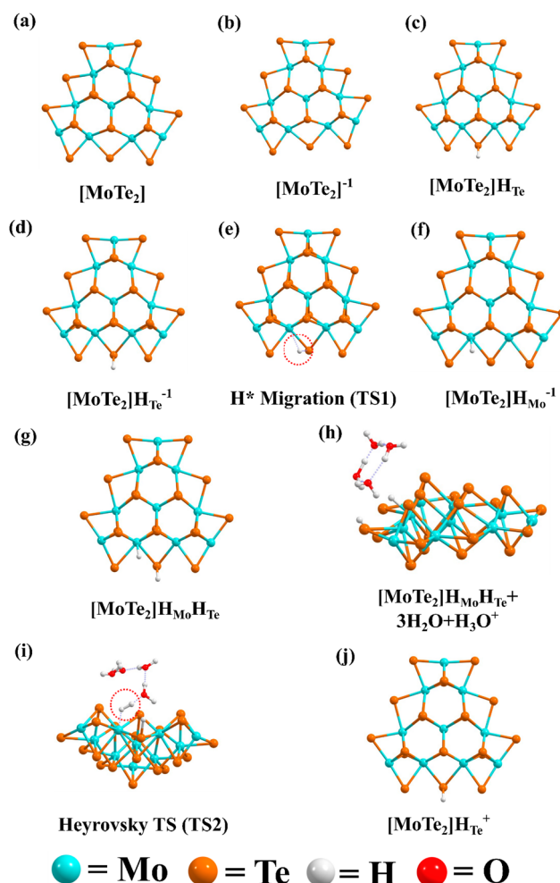
Fig. 4 The equilibrium geometry of important reaction intermediates and TSs: (a) [MoTe_2] , (b) [MoTe_2]^-1 , (c) [MoTe_2]H_{Te} , (d) [MoTe_2]H_{Te}^-1 , (e) H^* -Migration TS (TS1), (f) [MoTe_2]H_{Mo}^-1 , (g) [MoTe_2]H_{Te}H_{Mo} , (h) [MoTe_2]H_{Mo}H_{Te} + 3H_2O + H_3O^+ , (i) Heyrovsky TS (TS2) and (j) [MoTe_2]H_{Te}^+ by M06-L calculation shows the DFT method considering the molecular cluster model system Nb_1Mo_9Se_{21} to represent the 2D monolayer of Nb–MoSe 2 .
