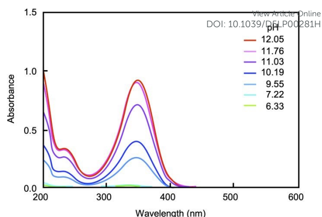
Fig. 10 UV absorbance of DSBP released from L-PAAm-DSBP composites at different pH values.
