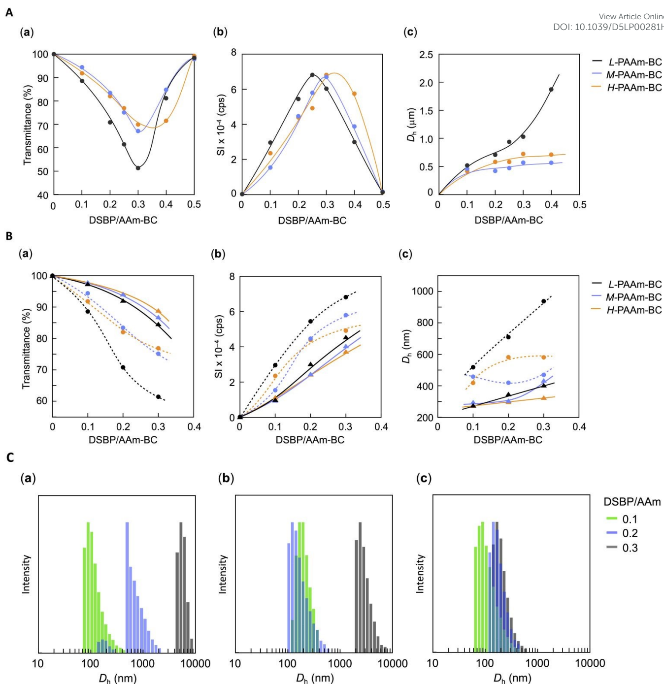
Fig. 4 (A) Variations in (a) transmittance, (b) scattering intensity and (c) hydrodynamic diameter of DSBP-captured PAAm-BC as a function of the DSBP/AAm-BC ratio. [\text{AAm-BC}]_0 = 3.57 \times 10^{-3} \text{ mol L}^{-1} . (B) Variations in (a) transmittance, (b) scattering intensity and (c) hydrodynamic diameter of DSBP-captured PAAm-BC as a function of the DSBP/AAm-BC ratio. [\text{AAm-BC}]_0 = 3.57 \times 10^{-3} \text{ mol L}^{-1} (dashed line) and 1.78 \times 10^{-3} \text{ mol L}^{-1} (solid line). (C) Weight conversion distributions in light scattering for (a) L-PAAm-BC, (b) M-PAAm-BC and (c) H-PAAm-BC at DSBP/AAm = 0.1, 0.2 and 0.3. [\text{AAm-BC}]_0 = 1.78 \times 10^{-3} \text{ mol L}^{-1} .
