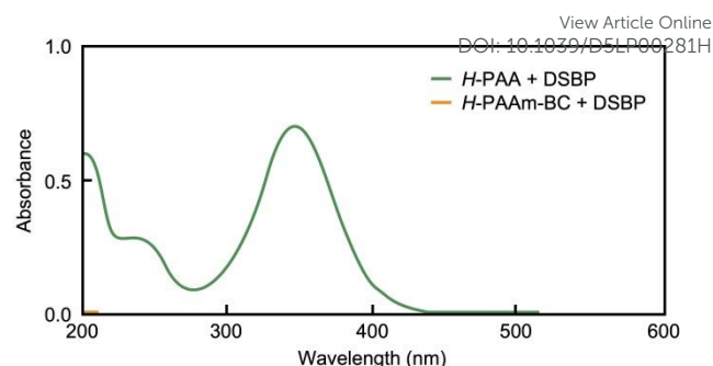
Fig. 3 UV spectra of the DSBP–PAA and DSBP–PAAm-BC mixtures. DSBP/AAm = DSBP/AA = 0.5. [AA]_0 = [AAm-BC]_0 = 3.57 \times 10^{-3} \text{ mol L}^{-1} .
