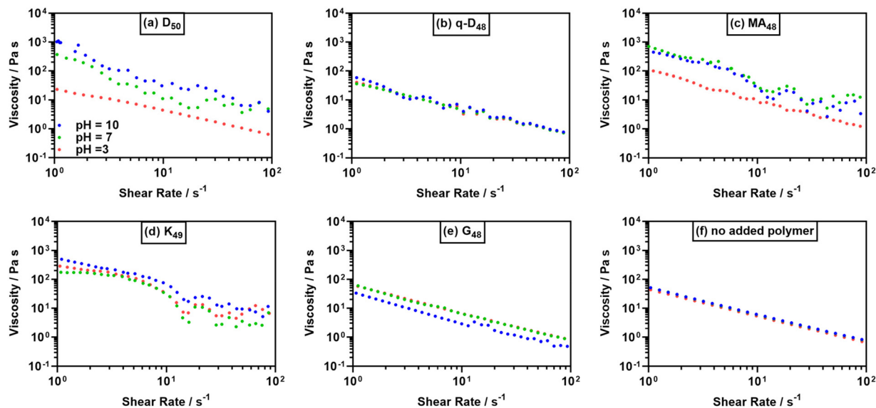
Fig. 4 Viscosity vs. shear rate for 50% w/w IOP suspensions with 0.5% w/w (a) D_{50} , (b) q\text{-}D_{48} , (c) MA_{48} , (d) K_{49} , (e) G_{48} , and (f) without added polymer at pH = 3 (red dots), pH = 7 (green dots) and pH = 10 (blue dots). The 0.5% w/w polymer additive concentration is based on IOP concentration.
