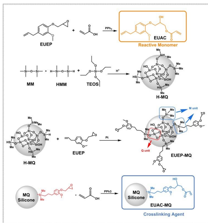
Fig. 2 Synthesis of EUAC and EUAC-MQ.
