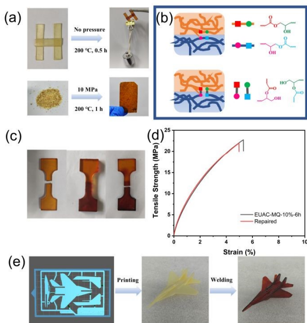
Fig. 7 Repairing and 3D printing: (a) Welding and recycle test; (b) Illustration of the reprocessing process; (c) Photos of the repaired samples; (d) Tensile curves of the repaired samples; (e) 2D plane model & the assembled plane model.
