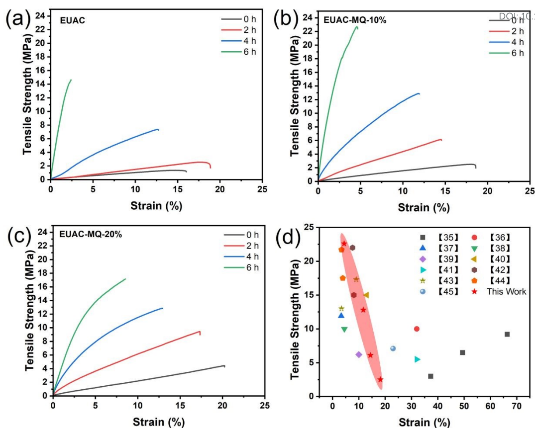
Fig. 5 Tensile curves of specimens cured at 180 °C for different times (a) EUAC; (b) EUAC-MQ-10%; (c) EUAC-MQ-20%; (d) literature-reported bio-based UV-cured resins tensile properties.
