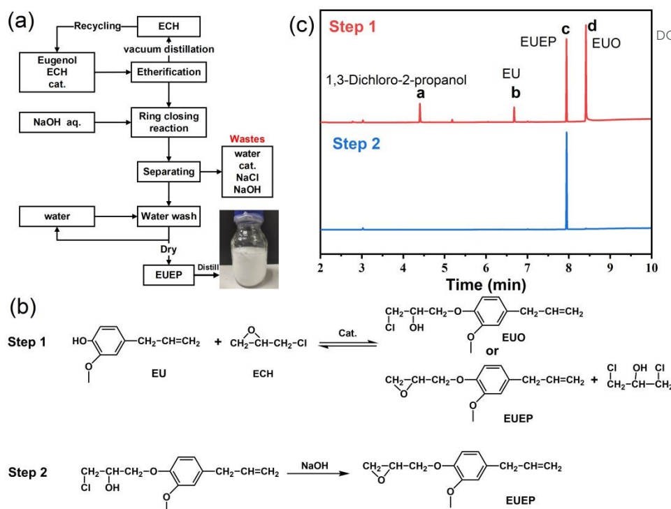
Fig. 1 (a) EUPE pilot test procedure, (b) Synthesis of EUPE, (c) GC spectra of two steps products.
