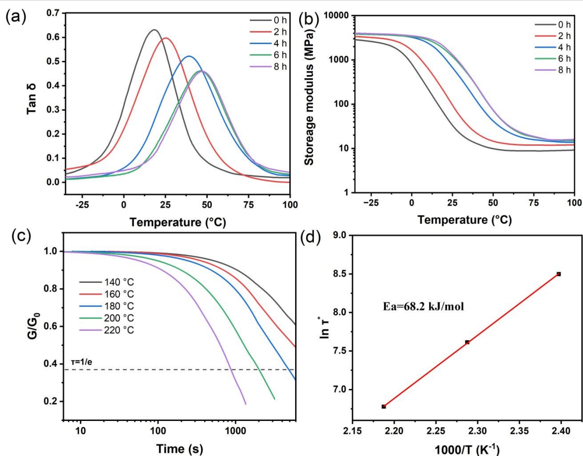
Fig. 6 DMA properties of EUAC-MQ-10% at 180 °C in different times (a) Tan \delta ; (b) Storage Modulus; Normalized stress–relaxation curves (c) and Arrhenius fitting line (d) of EUAC-MQ-10% at different temperatures.
