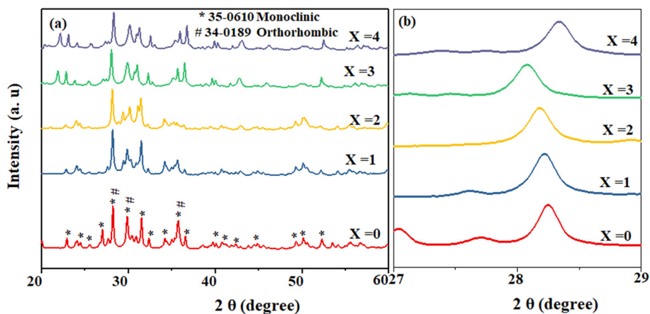
Fig. 2 XRD results of MCSZO- X ( X = 0-4 ) nanoparticles. (a) XRD patterns of different samples of MCSZO ( X = 0-4 ), calcined at 1300\ \text{°C} for 10 h. (b) Enlarged view of the highest intense peaks of samples.
