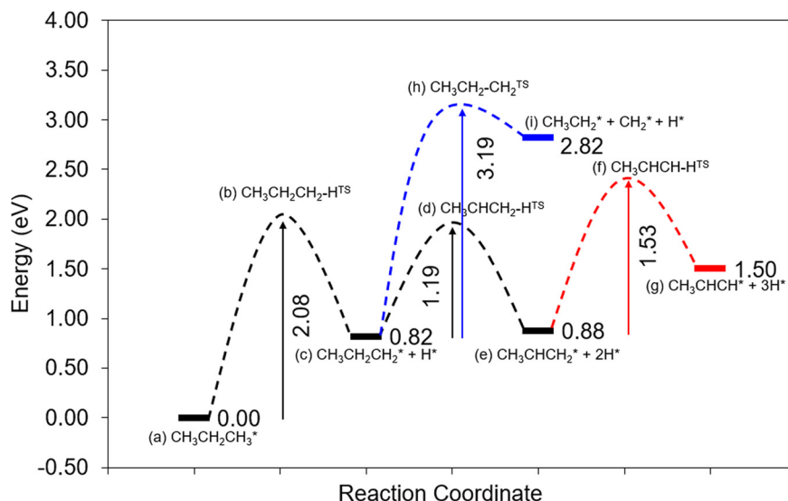
Fig. 6 Energy diagram from propane dehydrogenation to propylene (black colour), propylene dehydrogenation (red colour) and C-C bond cleavage of the CH 3 CH 2 CH 2 intermediate (blue colour).
