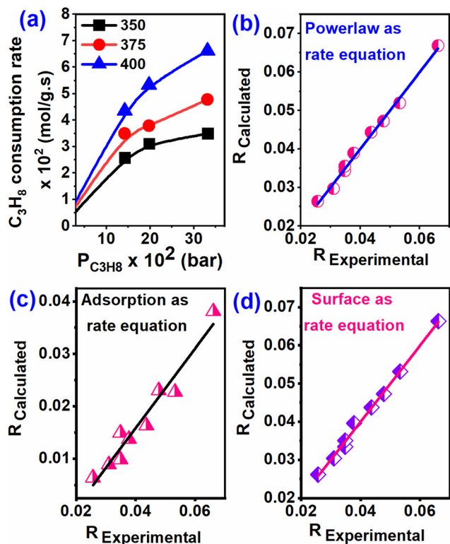
Fig. 5 (a) Dependence of the rates of C 3 H 8 consumption over Cu-TiO 2 measured at 350, 375, and 400 °C on the C 3 H 8 partial pressure. (b–d) Plot of R calculated vs. R observed of the data taken between 350 and 400 °C.
