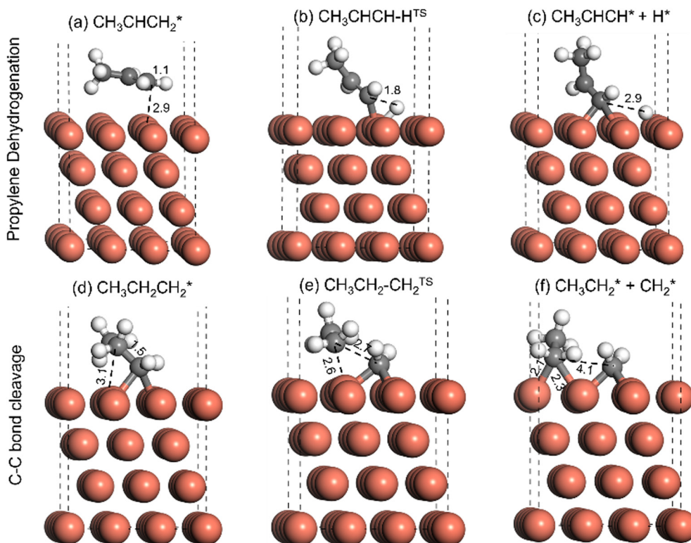
Fig. 7 DFT optimized geometry for adsorbates and TS during (a-c) propylene dehydrogenation and (d-f) C-C bond cleavage of the adsorbed CH 3 CH 2 CH 2 intermediate.
