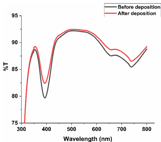
Fig. 5 UV-vis spectra for Ni 2+ ion presence in nickel standard solution before and after 2-hour electrodeposition at pH 3.5 and 60 °C.
