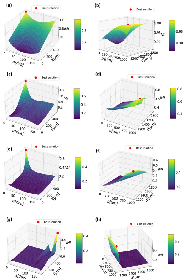
Fig. 7 3D surface plot of MI for four-parameter optimization of the micromixer with parallelogram barriers with labeled optimal solution proposed by BO. (a) Angle of barrier inclination \alpha and barrier height l , Re = 1; (b) barrier width p and distance between barriers d , Re = 1; (c) angle of barrier inclination \alpha and barrier height l , Re = 5; (d) barrier width p and distance between barriers d , Re = 5; (e) angle of barrier inclination \alpha and barrier height l , Re = 10; (f) barrier width p and distance between barriers d , Re = 10; (g) angle of barrier inclination \alpha and barrier height l , Re = 100; (h) barrier width p and distance between barriers d , Re = 100.
