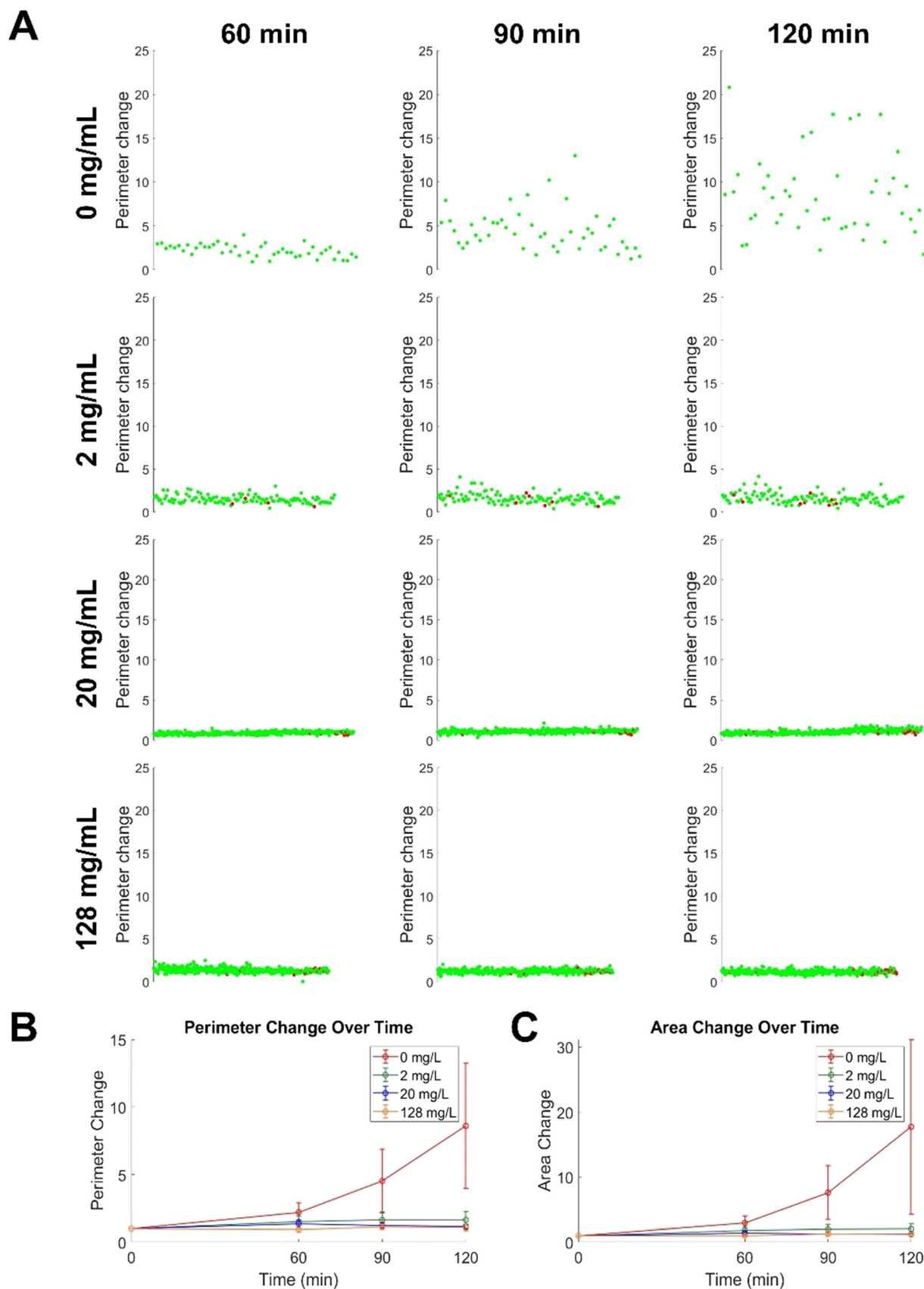
Fig. 7 Single cell response kinetics to different concentrations of ciprofloxacin. (A) Normalized changes in the perimeter of individual bacteria at 60, 90, and 120 min. The bacteria were inoculated at 0, 2, 20, and 128 mg L -1 of ciprofloxacin dissolved in MHB at 37 °C. Values were normalized to the initial measurement. Red dots indicate dead cells as shown by PI staining. Values were normalized to the initial measurement. (B and C) Growth kinetics of bacterial perimeter and area. Values were normalized to the initial measurement.
