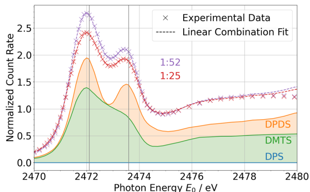
Fig. 4 NEXAFS spectra of a mixture of DPS, DPDS and DMTS in a volumetric mixing ratio of 0 : 8 : 2 (no DPS), measured at the MiFo beamline in fluorescence mode. Experimentally acquired spectra are shown with crosses; the linear combination fit results are plotted with dashed lines. The samples were diluted with n -dodecane in ratios of 1 : 25 (red) and ca. 1 : 52 (purple). The shape of the spectra and the composition of the sample are reproduced by the linear combination analysis which was performed simultaneously for both different levels of dilution including self-absorption correction. The contributions of the basis spectra of DPS (blue), DPDS (orange) and DMTS (green) are indicated in their respective colours.
