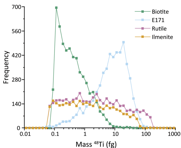
Fig. 1 Mass distributions of 48 Ti in the pristine suspensions of biotite, E171, rutile, and ilmenite.
