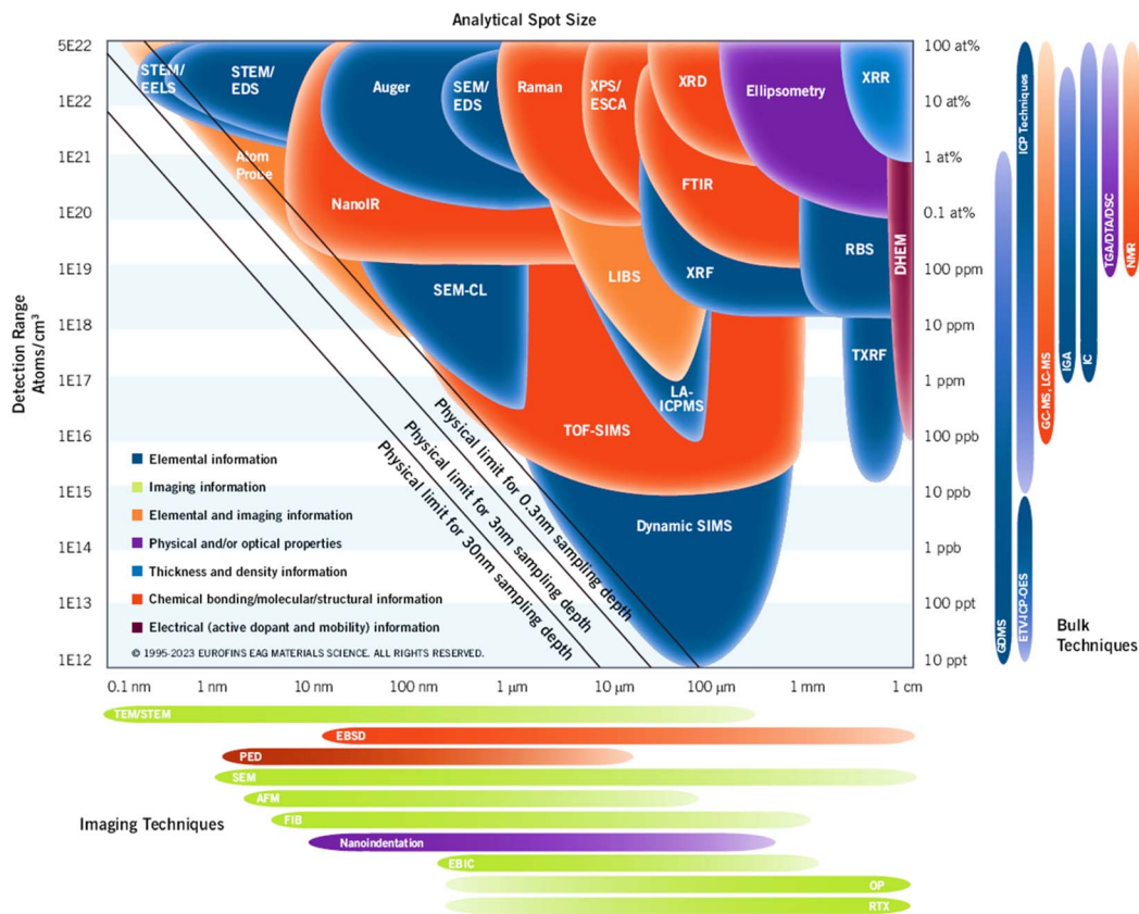
Fig. 3 Analytical resolution, spot size, and detection limit of common characterization techniques (the data source comes from the EAG Laboratories website).
