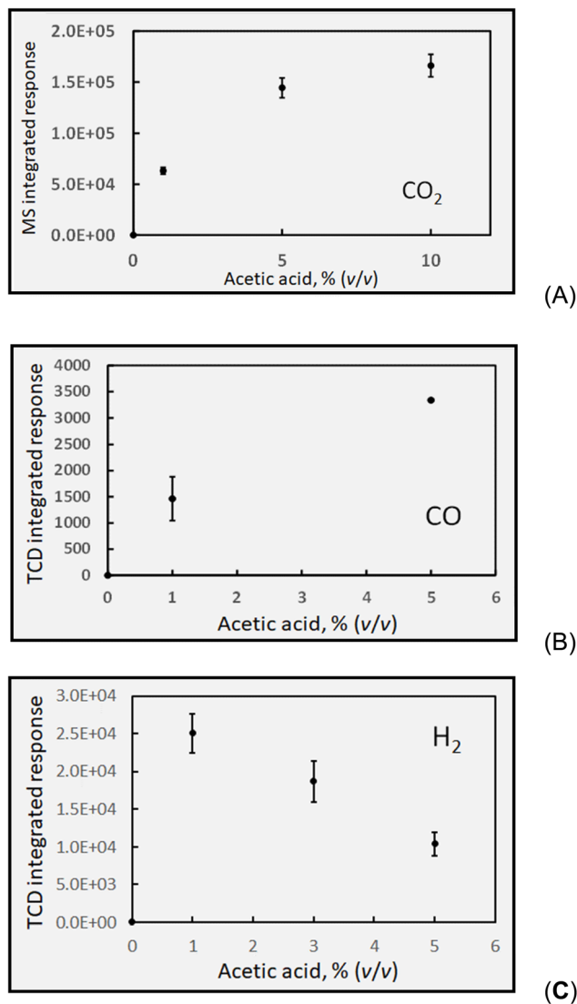
Fig. 5 Effect of acetic acid concentration on analyte gas response (generation) at 2 \text{ mL min}^{-1} solution flow rate ( t_{\text{IT}} = 22 \text{ s} ). (A) \text{CO}_2 production, uncorrected HS [\text{CO}_2] = 1730 \pm 30 \text{ ppm} (repeatability SD, n = 4 ) at 5% (v/v) acetic acid. (B) CO production, uncorrected HS [\text{CO}] = 14 \pm 4 \text{ ppm} (repeatability SD, n = 9 ) at 5% (v/v) acetic acid. (C) \text{H}_2 production, uncorrected HS [\text{H}_2] = 290 \pm 40 \text{ ppm} (repeatability SD, n = 3 ) at 5% (v/v) acetic acid. Ordinate displays integrated response characterizing chromatographic peaks.
