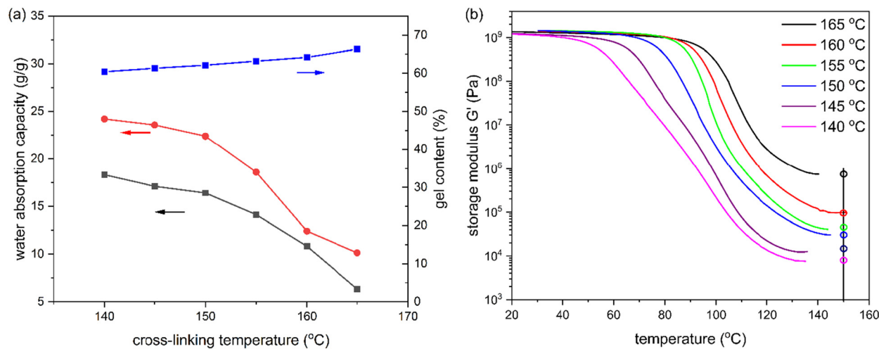
Fig. 2 (a) Water absorption capacity and gel content of SAPs (all variations of SAP-80) versus cross-linking temperature; (■) water absorption capacity of unextracted SAP-80s (ground for 180 s), (●) water absorption capacity of extracted SAP-80s (ground for 180 s); (■) gel content of extracted SAP-80s (ground for 180 s); note: all the data shown in the figure are average values based on the results obtained for three separate measurements and the margins of error are \pm 2 \text{ g g}^{-1} for the water absorption capacity test and \pm 0.2\% for the gel content test. (b) Storage modulus as a function of temperature of extracted SAP-80s cross-linked at different temperatures (140 °C to 165 °C) for 1 h versus temperature and ground for 180 s. Note: 150 °C (vertical black line) was chosen as the point where G_x was taken; since all curves reached a plateau before 150 °C, it is reasonable to predict the G' value according to the existing curve. The circles are the predicted point at 150 °C.
