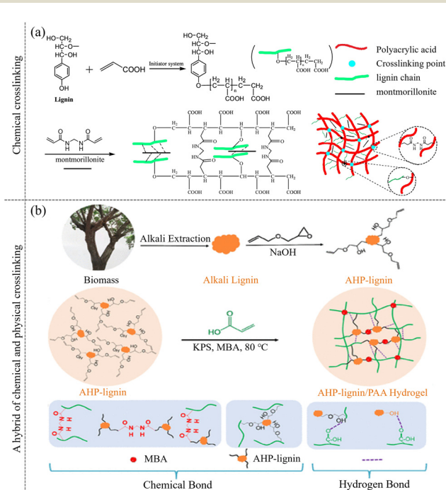
Fig. 5 Chemical and physical crosslinking of lignin-based hydrogels. 110,115 (a) The preparation diagram of a composite hydrogel by combining lignin and montmorillonite. [Reproduced from ref. 110 with permission from Elsevier, copyright of 2019.] (b) Preparation of AHP-lignin/PAA hydrogel. [Reproduced from ref. 115 with permission from American Chemical Society, copyright of 2022.]
