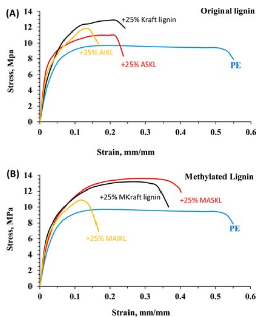
Figure 16. Comparison of the stress vs. strain curves for SKL - polyethylene blends. Polyethylene blends were obtained for both unmodified (up) and methylated (down) lignin/fractions. Reproduced from reference 169 with permission from American Chemical Society, copyright 2016.
