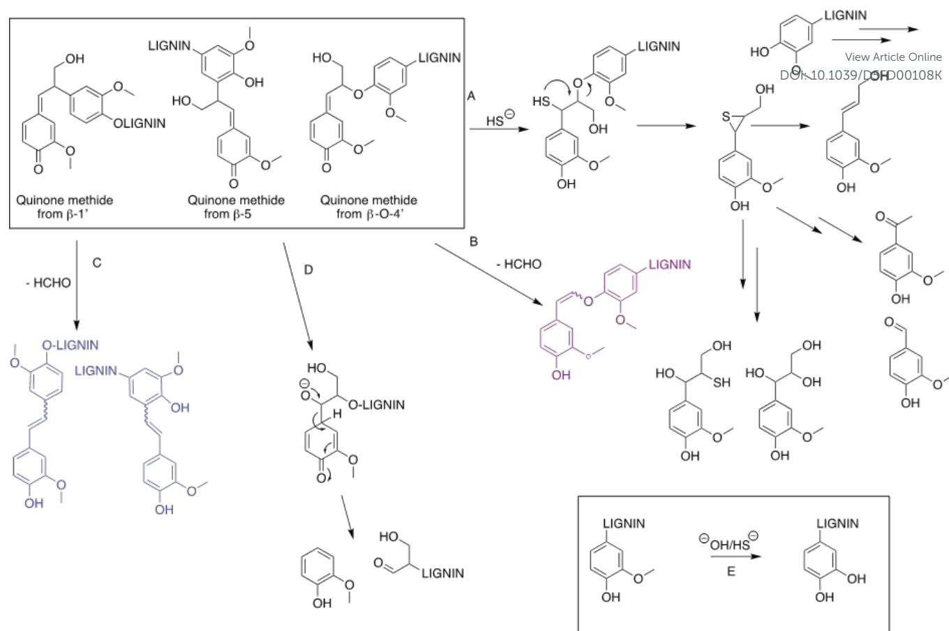
Figure 3. Key reactions from quinone methide intermediates during kraft pulping. Reproduced from reference 5 with permission from Wiley, copyright 2023.
