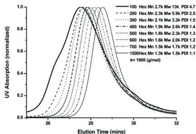
Figure 6. Size-exclusion chromatograms of SKL fractions isolated via fractional precipitation. 8 Reproduced from reference 38 with permission from American Chemical Society, copyright 2014..
