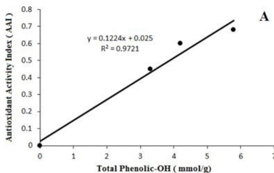
Figure 13. Correlation of phenolic hydroxyl groups content with the antioxidant activity index of SKL and its fractions. Reproduced from reference 168 with permission from American Chemical Society, copyright 2015..
