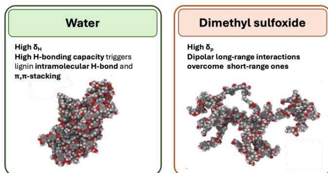
Figure 10. A molecular simulation of lignin conformation in water and DMSO, respectively, has been reported. 93 The high hydrogen-bonding parameter ( \delta_H ) of water, indicative of strong short-range hydrogen bonding, enhances intramolecular \pi - \pi stacking and hydrogen bonds within lignin, thereby promoting a collapsed molecular configuration. In contrast, the high polarity parameter ( \delta_P ) of DMSO facilitates extended dipolar interactions between lignin and the solvent, favoring an elongated conformation. Reproduced from reference 72 with permission from Nature, copyright 2024..
