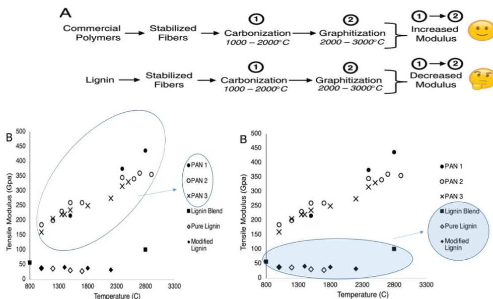
Figure 21. (A) Schematic conveying an overlooked discrepancy in the temperature–modulus relationship among lignin-derived and commercial carbon fibers. (B) Plots showing the change in tensile modulus as a function of temperature for six carbon fibers (adapted from 182–186 ). PAN 1, 2, & 3 refer to Polyacrylonitrile carbon fibers treated at 1000–2900 °C, 182–186 To the right of Fig 21 Lignin Blend data is shown: Carbon fibers derived from pyrolysis fuel oil blended with hardwood kraft lignin treated at 800 and 2800 °C, 185 Pure Lignin: Carbon fibers derived from SKL treated at 1000–1700 °C, 184 Modified Lignin: Carbon fibers derived from acylated softwood lignin treated at 1000–2200 °C. 186 Reproduced from reference 180 with permission from Royal Society of Chemistry, copyright 2019. .
