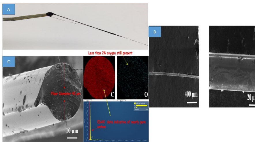
Figure 20. (A) Showing fibers being pulled out of the melt from methylated/propargylated softwood kraft lignin; (B) photo-micrographs of fibers after carbonization; (C) Cross-section & EDAX analyses of carbon fibers produced from methylated/propargylated SKL.
