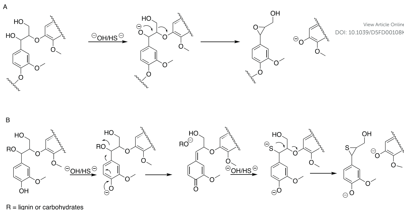
Figure 2. Cleavage of non-phenolic and phenolic \beta -O-4 bonds during kraft pulping. A: slow sulphur-independent reaction, endo-depolymerisation; B: fast sulphur-dependent reaction, exo-depolymerisation. 7,8 Reproduced from reference 5 with permission from Wiley, copyright 2023..
