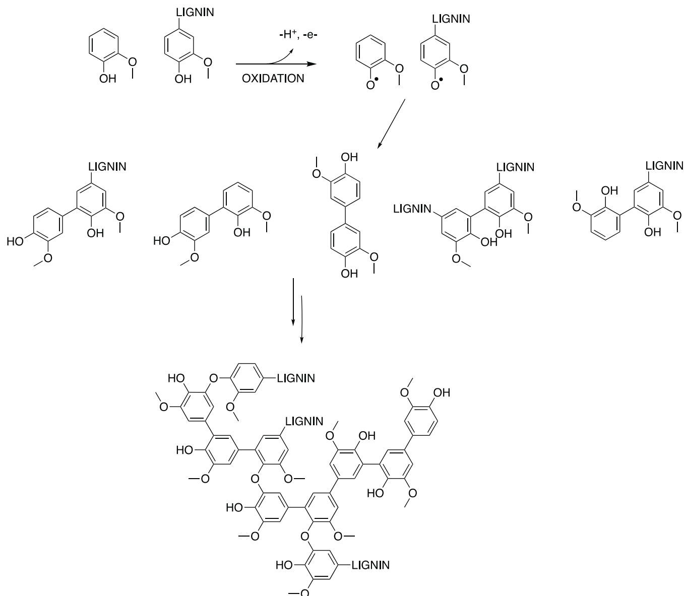
Figure 4. Possible radical oxidative coupling modes of lignin fragments released during kraft pulping. 8 Reproduced from reference 16 with permission from Royal Society of Chemistry, copyright 2017..
