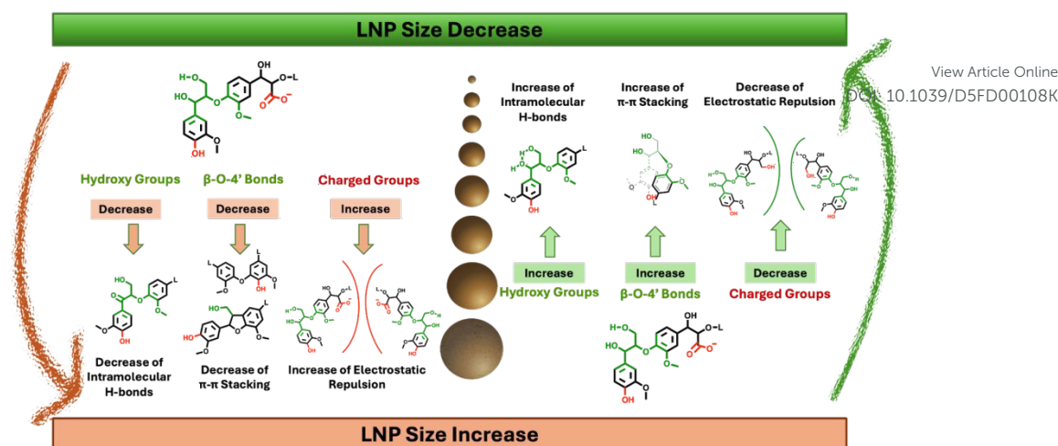
Figure 12. The size of lignin nanoparticles is influenced by several structural characteristics. A high concentration of hydroxyl groups promotes extensive intramolecular hydrogen bonding, which in turn leads to a more compact lignin conformation and the formation of smaller nanoparticles. Similarly, a greater abundance of β-O-4 linkages enhances π-π stacking interactions, also resulting in smaller particle sizes. The stronger π-π interactions associated with guaiacyl (G) units, as compared to syringyl (S) units, favour the production of smaller particles from softwood lignin. In contrast, the presence of charged groups—such as carboxylates—increases electrostatic repulsion between molecules, thereby encouraging the formation of larger particles. The dependence of lignin particle size on molecular weight is primarily attributed to variations in the distribution of aliphatic and phenolic hydroxyl groups across different lignins or lignin fractions. 132,136,138,144 Reproduced from reference 72 with permission from Nature, copyright 2024.
