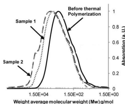
Figure 18. Weight average molecular weight distributions of the methylated/ propargylated SKL before and after the thermally-induced polymerization. Samples 1 and 2 were polymerized at 150°C, for 10 and 60 minutes respectively. Reproduced from reference 179 with permission from American Chemical Society, copyright 2013.
