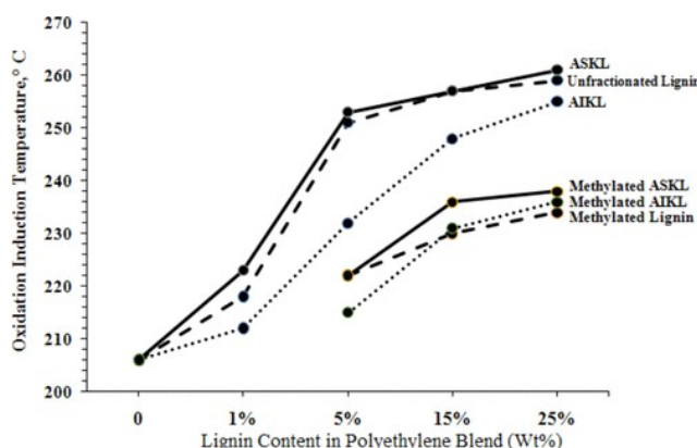
Figure 14. Correlation of lignin content (unfractionated SKL and its fractions) in PE-blends with the OI_{temp} . Reproduced from reference 168 with permission from American Chemical Society, copyright 2015.
