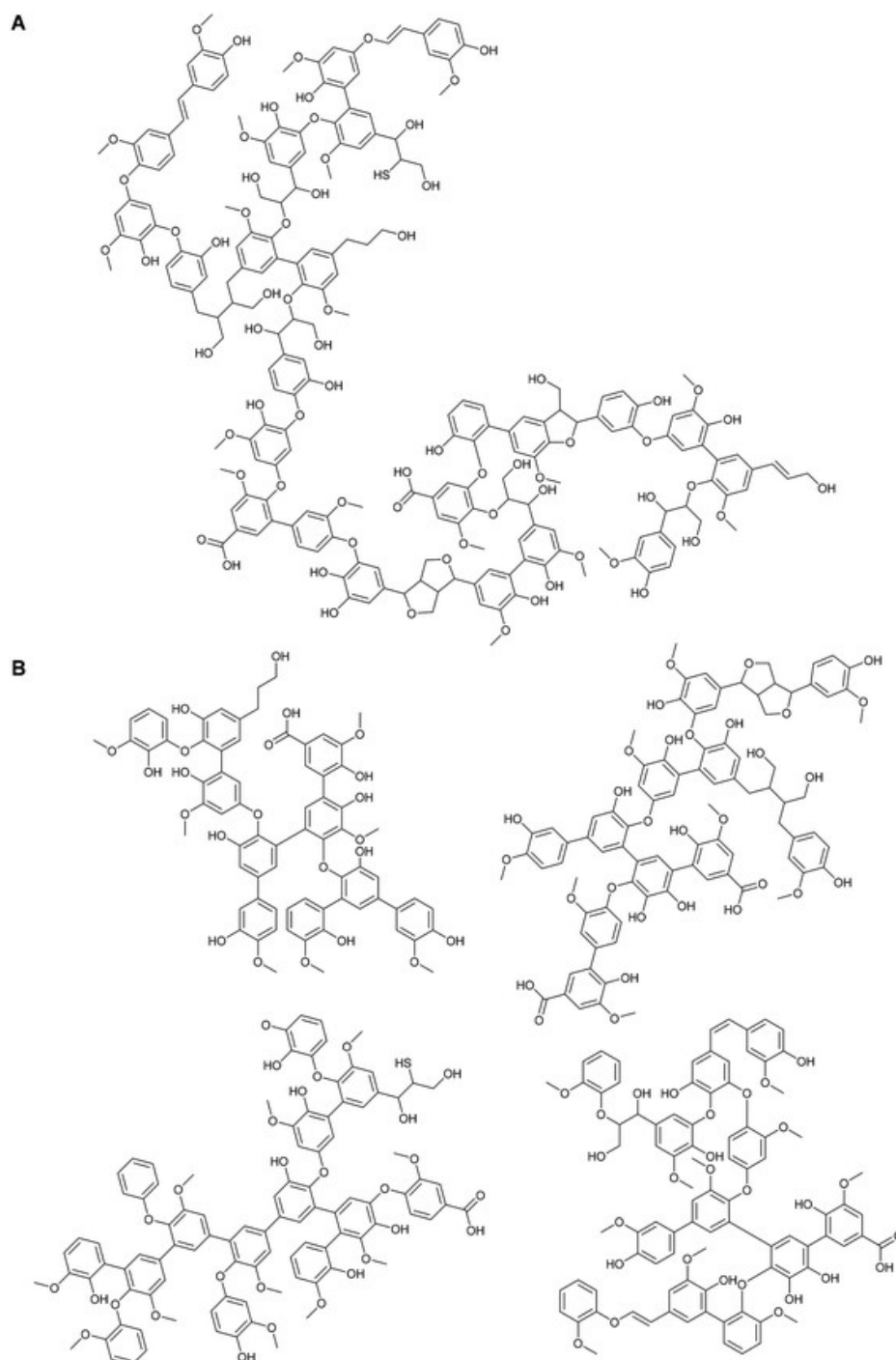
Figure 5. Proposed new structure for Softwood Kraft lignin (SKL) composed of a mixture of: (A) Large lignin segments containing some native lignin structures; (B) Smaller lignin segments enriched with phenolic character. 8 Reproduced from reference 16 with permission from Royal Society of Chemistry, copyright 2017.
