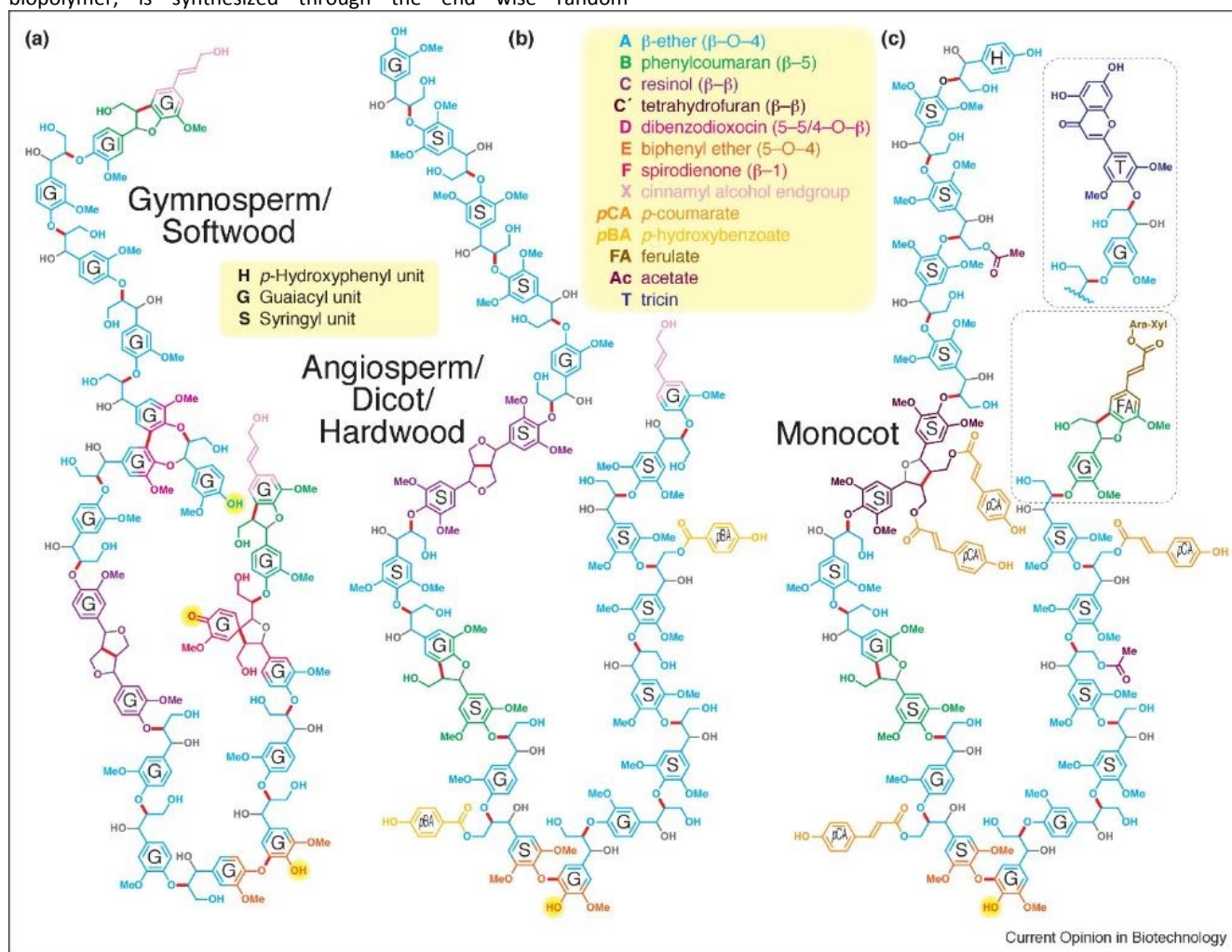
Figure 1. Current lignin structure according to Ralph, Lapierre, and Boerjan. 4 Reproduced from reference 4 with permission from Elsevier, copyright 2019.
