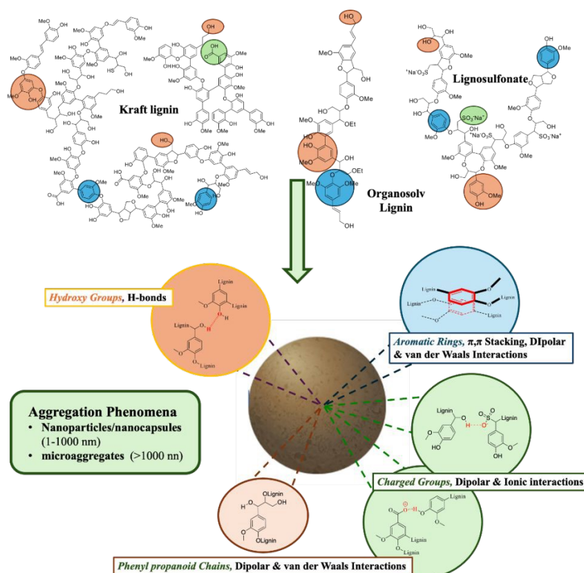
Figure 9. Sites for inter/intramolecular association highlighted in technical lignins. 8 Reproduced from reference 72 with permission from Nature, copyright 2024..
