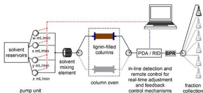
Figure 8. Schematic flow scheme of SCFF for lignins, with facultative, eventually PC-controlled column exchange mechanism for scale-up. 8 Reproduced from reference 70 with permission from Wiley, copyright 2020..
