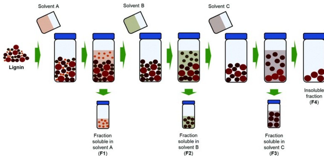
Figure 7. Sequential solvent extraction. 8 Reproduced from reference 39 with permission from Royal Society of Chemistry, copyright 2020.
