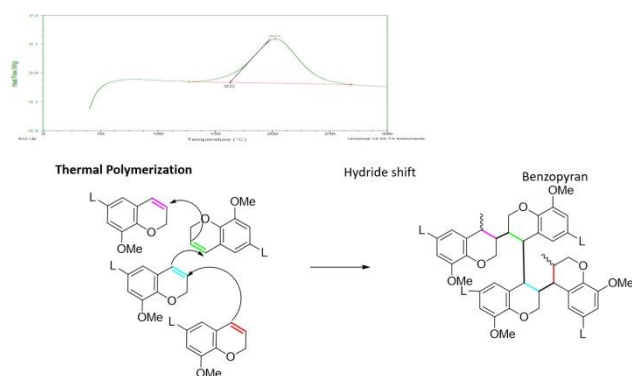
Figure 19. Differential Scanning Calorimetry offers a convenient means to monitor the degree of thermal polymerization of the propargylated SKL by evaluating the developed exotherm depicted.
