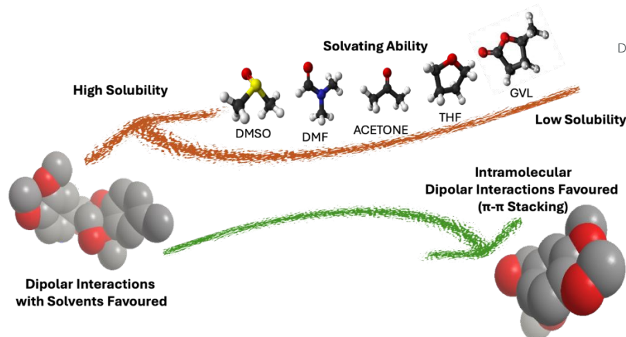
Figure 11. As the solvating power of various solvents increases (left), dipolar interactions between lignin and the solvent are increasingly favored. Conversely, in solvents with lower solvating efficiency, intramolecular \pi - \pi stacking and hydrogen bonding within the lignin structure, dominate. Under such conditions, lignin adopts a more compact conformation in solution, and the subsequent introduction of water as an antisolvent promotes the formation of nanoparticles (right). Reproduced from reference 72 with permission from Nature, copyright 2024..
