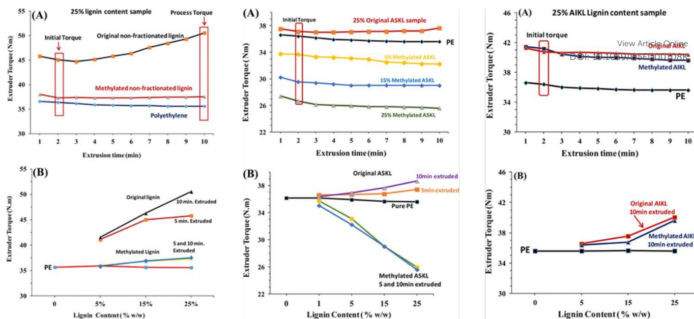
Figure 15. Comparison of the extruder torque for SKL–polyethylene blends at different lignin loadings with SKL (left), ASKL (centre), and AIKL (right). Reproduced from reference 169 with permission from American Chemical Society, copyright 2016.
