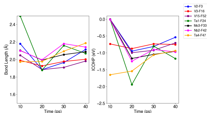
Fig. 7 Bond length and integrated crystal orbital Hamiltonian population (ICOHP) of metal fluorides at the (100)NbTaMoWV-FLiBe interface at 800 K. The cutoff distance for the atom pair is 3 Å. If the distance between the atom pair exceeds 3 Å, the interatomic interaction is considered insignificant and the bond length and ICOHP are not reported.
