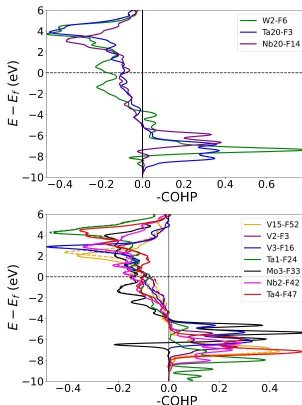
Fig. 8 Crystal orbital Hamiltonian population (COHP) analysis of the BCC (100) surfaces of NbTaMoW and NbTaMoWV in contact with molten FLiBe, evaluated at 800 K after 40 ps of simulation time. The black dotted line represents the Fermi level which is set to 0 eV.
