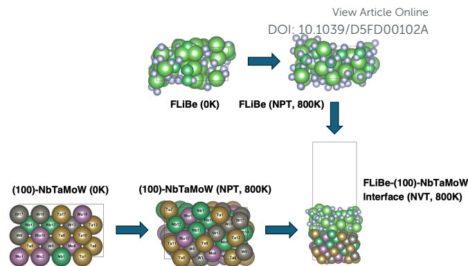
Fig. 1 Workflow for constructing the Refractory High Entropy Alloy (RHEA)-FLiBe interface. Top left: Initial configuration of FLiBe at 0 K. Top right: Thermally equilibrated FLiBe at 800 K under NPT conditions. Bottom left: Initial BCC (100) NbTaMoW slab at 0 K. Bottom middle: Thermally relaxed BCC (100) NbTaMoW at 800 K under NPT ensemble. Bottom right: Construction of the interface between the equilibrated BCC slab and molten salt, for under NVT conditions at 800 K.
