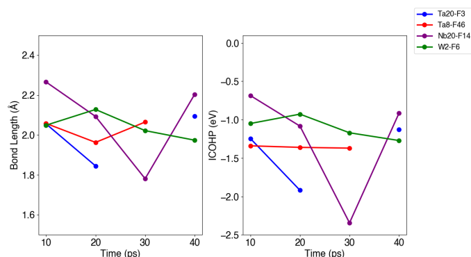
Fig. 6 Bond length and integrated crystal orbital Hamiltonian population (ICOHP) of metal fluorides at the (100)NbTaMoW-FLiBe interface at 800 K. The cutoff distance for the atom pair is 3 Å. If the distance between the atom pair exceeds 3 Å, the interatomic interaction is considered insignificant and the bond length and ICOHP are not reported.
