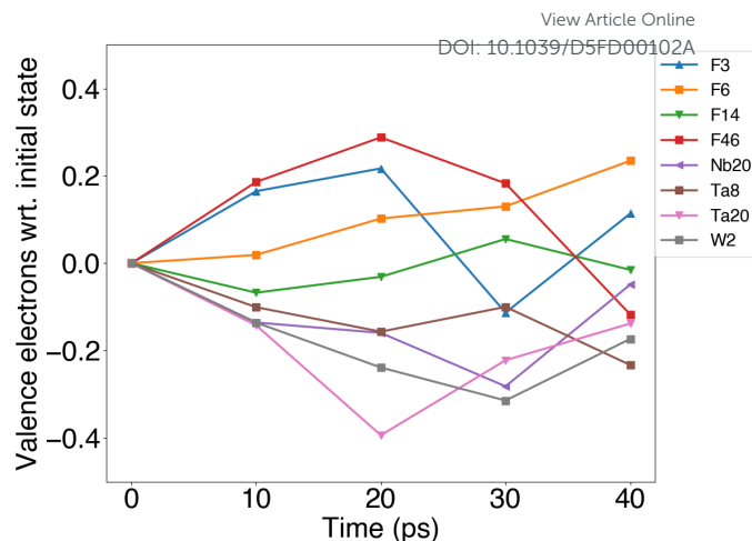
Fig. 9 Change in valence electrons of surface atoms at the interface between (100)-NbTaMoW and FLiBe at 800 K. The number of valence electrons for a given atom is normalized to the valence electrons at 0 ps.
