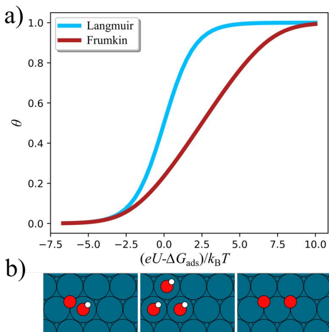
Figure 1 a) Coverage, \theta , as function of potential, U , (or chemical potential). The Langmuir isotherm model in blue, \theta = \left(1 + \exp\left(-\frac{eU - \Delta G_{ads}}{k_B T}\right)\right)^{-1} , where \Delta G_{ads} is the adsorption free energy. The Frumkin isotherm model in red, \theta = \left(1 + \exp\left(-\frac{eU - \Delta G_{ads} - \alpha\theta}{k_B T}\right)\right)^{-1} , where \alpha is the adsorbate-adsorbate interaction term. The plot uses \alpha = 5k_B T . b) Examples of local *OH-O* , *OH-*OH , and O*-O* adsorption configurations that could be disallowed by the blocking rules.
