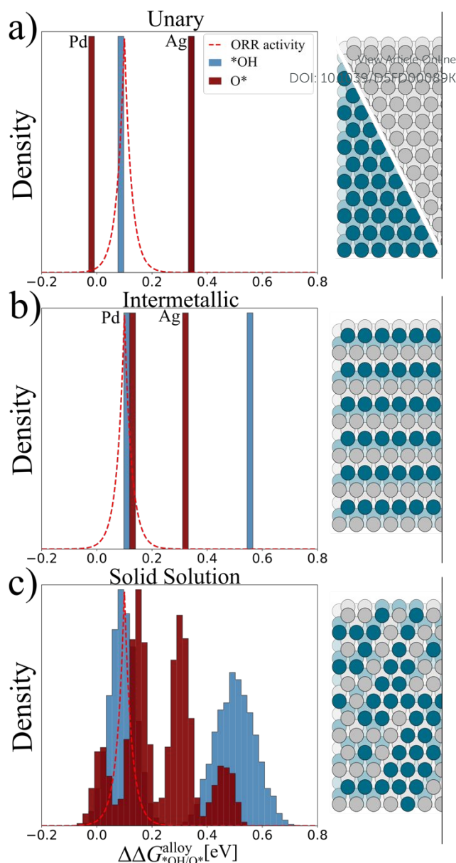
Figure 2. Gross \ast\text{OH} / \text{O}^\ast adsorption energy distributions and illustration of the atomic configurations at the surface for a) unary Pd(111) or Ag(111), b) intermetallic PdAg(111), and c) equimolar solid solution PdAg(111). In a) and b) it is indicated which O binding energy correspond to which metal.
