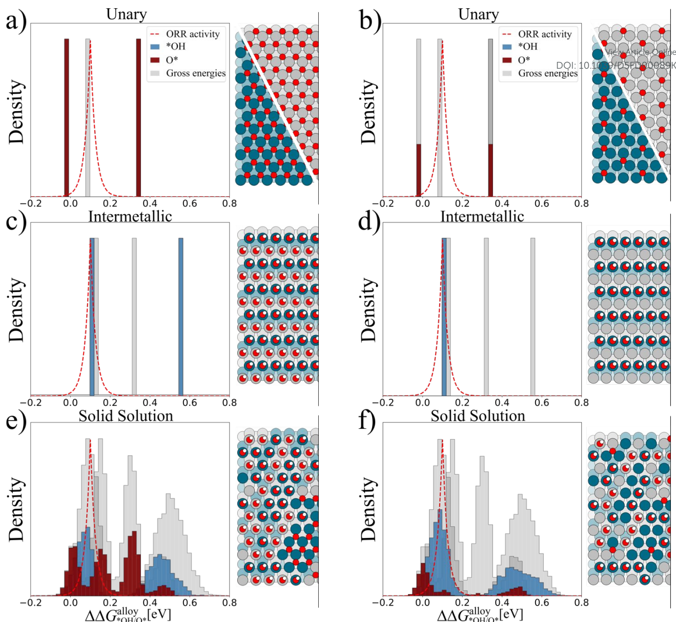
Figure 5. Left column shows gross (grey background) and net (full colour) ^*\text{OH} / \text{O}^* adsorption energy distributions and illustration of the adsorbate coverage when the adsorbates are blocking according to the mutual blocking rules for a) unary Pd(111) or Ag(111), c) intermetallic PdAg(111), and e) equimolar solid solution PdAg(111). Right column shows gross (grey background) and net (full colour) ^*\text{OH} / \text{O}^* adsorption energy distributions and illustration of the adsorbate coverage when the adsorbates are blocking in accordance with the extended blocking scheme for b) unary Pd(111) or Ag(111), d) intermetallic PdAg(111), and f) equimolar solid solution PdAg(111).
