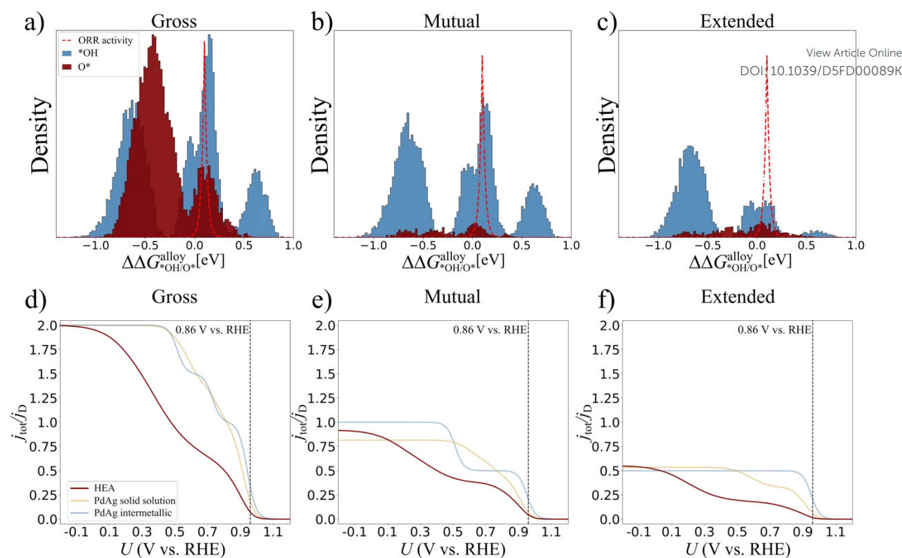
Figure 7. \text{Ag}_{14}\text{Ir}_{16}\text{Pd}_{30}\text{Pt}_{14}\text{Ru}_{26} HEA (111) surface a) gross ^*\text{OH} / \text{O}^* adsorption energy distributions and net ^*\text{OH} / \text{O}^* adsorption energy distributions obtained with b) mutual blocking or c) extended blocking rules. Potential dependent ORR current of the PdAg intermetallic, the equimolar PdAg solid solution, and the \text{Ag}_{14}\text{Ir}_{16}\text{Pd}_{30}\text{Pt}_{14}\text{Ru}_{26} HEA given that either d) the gross distributions, e) mutual blocking net distributions, or f) extended blocking net distributions determine the ORR activity.
