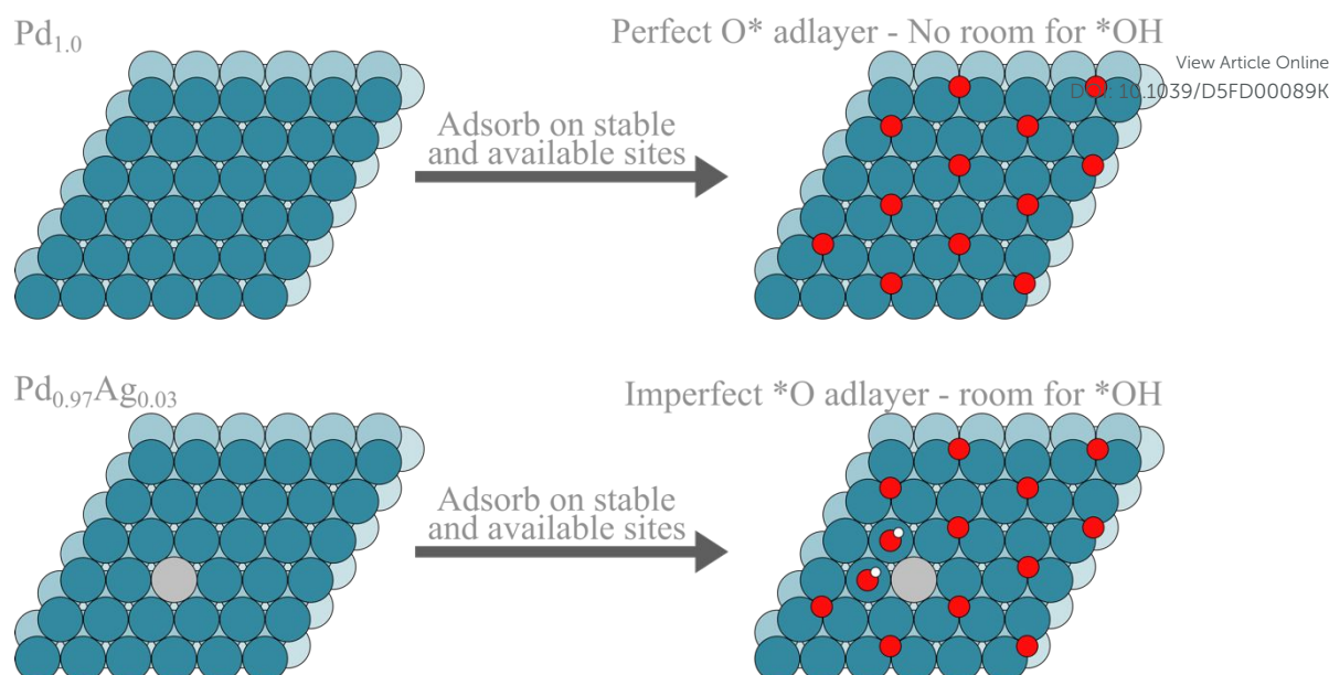
Figure 4 Coverage of adsorbed species using extended blocking rules for Pd(111) (top row) and Pd(111) with a single Ag atom (bottom row). The presence of *OH species in Pd(111) with a single Ag atom improves the ORR activity by one order of magnitude.
