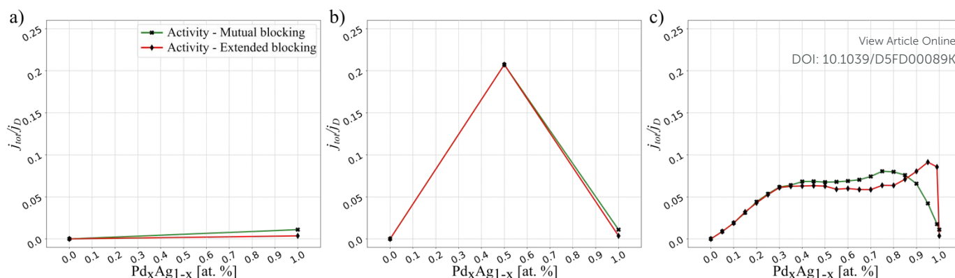
Figure 6 Predicted ORR activity at U = 0.86 V vs. RHE for a) unary surfaces, b) intermetallic, and c) solid solution as a function of Pd content in the alloy.
