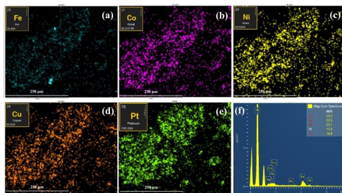
Fig. 2 (a–e) Elemental mapping images of uncapped FeCoNiCuPt HEA particles, and (f) its EDS spectra.
