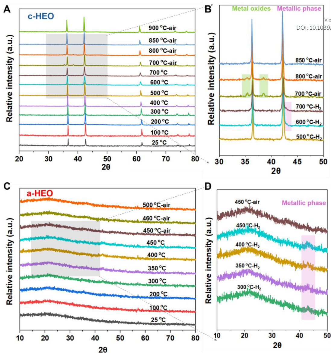
Figure 2 In situ XRD patterns of c-HEO (A, B) and a-HEO (C, D) collected at programmed temperatures under reducing (2% H 2 in He) and oxidative (air) atmosphere.
