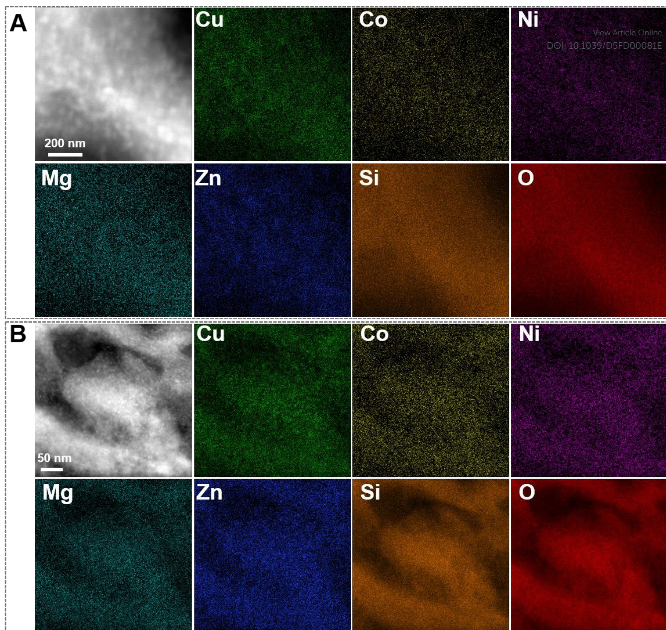
Figure 6 Microscopy of treated samples of a-HEO after reduction under 5% H 2 at 300 °C (A) and subsequent oxidation under air at 350 °C (B).
