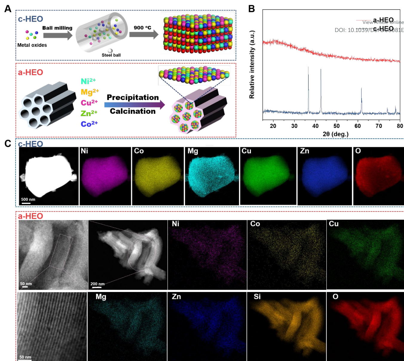
Figure 1 (A) Synthesis procedure and characterization of c-HEO and a-HEO by (B) XRD; (C) SEM, TEM, and elemental mapping.
