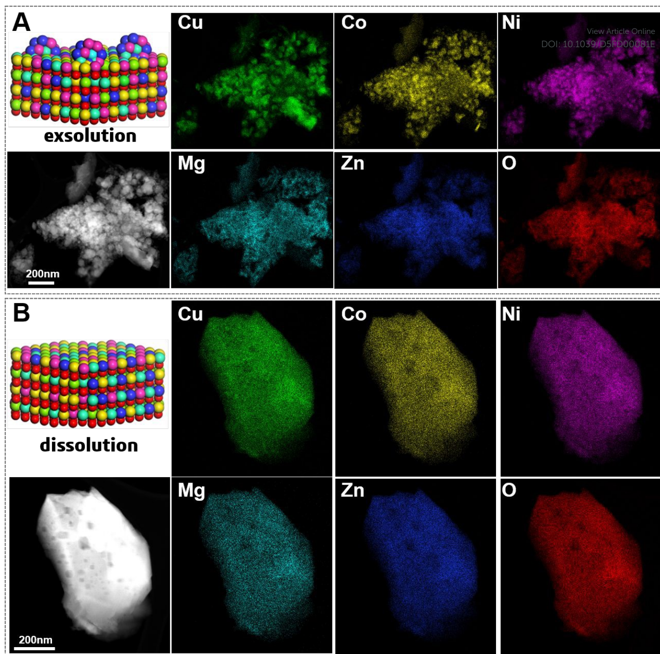
Figure 5 Microscopy of treated samples of c-HEO after reduction under 5% \text{H}_2 at 600 °C (A) and subsequent oxidation under air at 900 °C (B).
