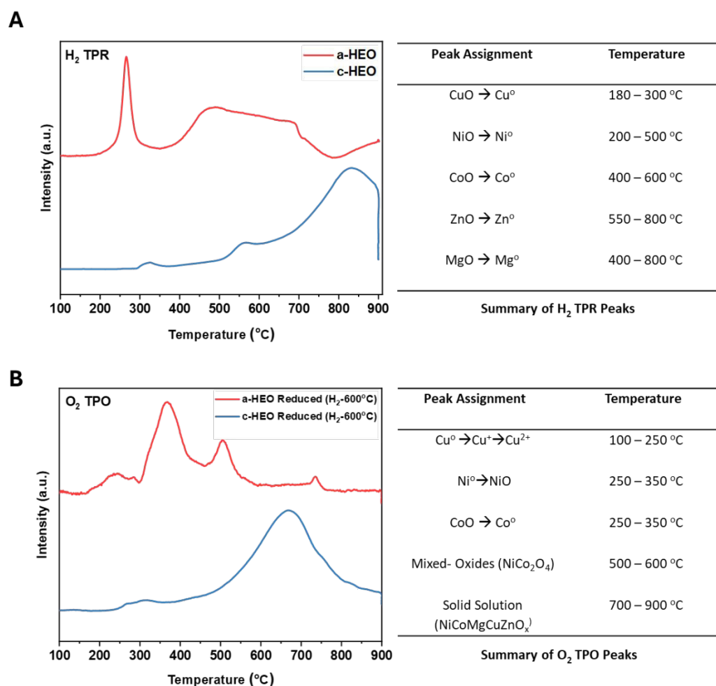
Figure 3 (A) H 2 TPR analysis of a-HEO and c-HEO with summary of H 2 TPR peaks; (B) O 2 TPO analysis of a-HEO reduced at 600°C in H 2 and c-HEO reduced at 600°C with summary of O 2 TPO peaks.
