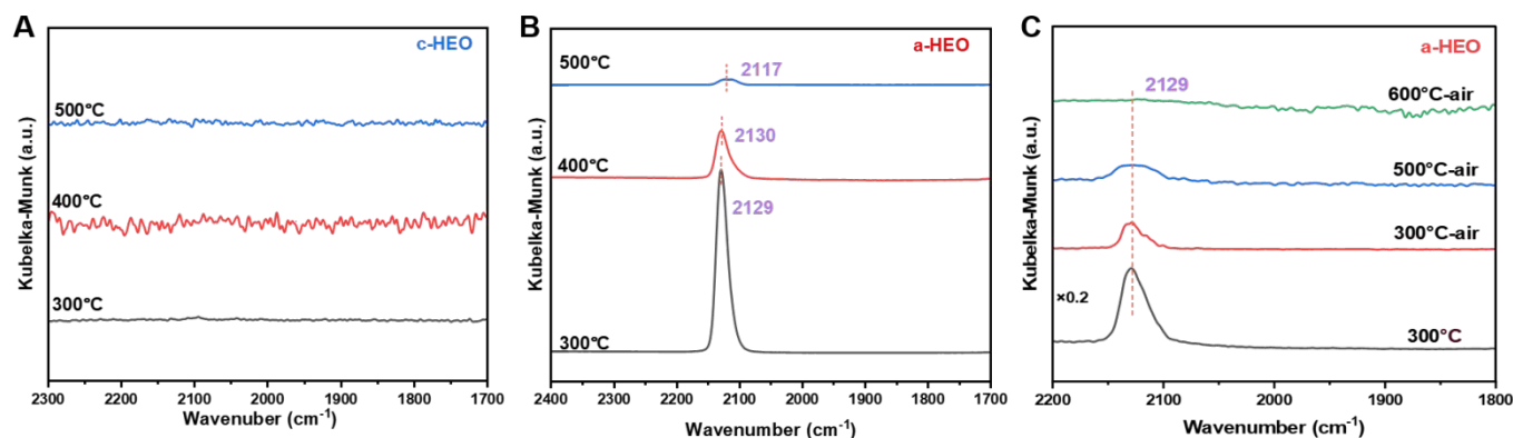
Figure 7 CO-DRIFTS results of c-HEO (A) and a-HEO (B) at different reduction temperatures under 5%H 2 /Ar atmosphere and a-HEO (C) at different oxidation temperatures under air atmosphere.
