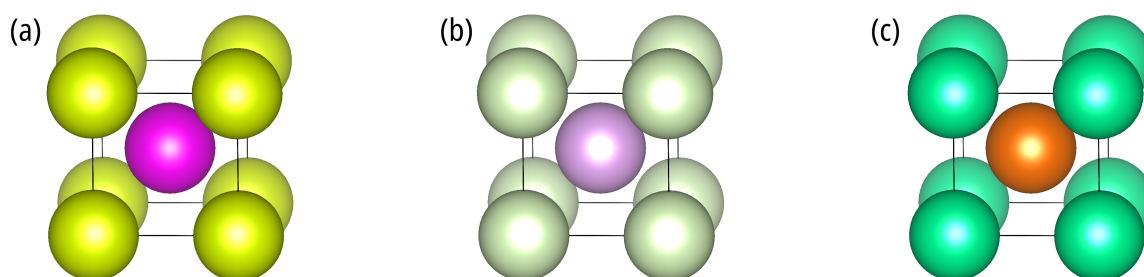
Fig. 2 Primitive cells of the quaternary B2 structures: (a) B2-I-(AlCr)-(TiV); (b) B2-II-(AlV)-(CrTi); (c) B2-III-(AlTi)-(VCr).
