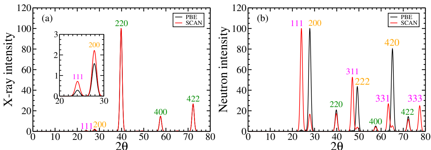
Fig. 5 X-Ray (a) and neutron (b) of structures simulated under PBE and SCAN exchange correlation functionals. Miller indexing is based on the 16-atom cubic cell of lattice constant 6.4 Å. Miller indices corresponding to a BCC (A2) lattice of lattice constant 3.2 Å are colored in dark green; B2 (CsCl) peak indices are orange; peaks unique to Heusler are magenta. Cu-K \alpha radiation ( \lambda = 1.5406 Å) is assumed for X-rays, and the same wavelength is chosen for the neutron pattern. The inset in (a) enlarges the vicinity of the (111) and (200) peaks.
