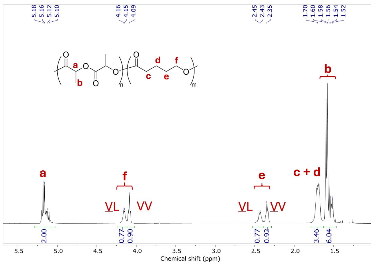
Figure 4: Assignment of the ^1\text{H} NMR spectrum of poly(lactide-co-valerolactone) copolymer prepared using 3 (Table 2, entry 12). V = valeroyl unit ( -\text{C}(\text{O})(\text{CH}_2)_4\text{O}- ), L = lactyl unit ( -\text{C}(\text{O})(\text{CH}(\text{CH}_3)\text{O}- ), LL = lactidyl unit ( -\text{C}(\text{O})(\text{CH}(\text{CH}_3)\text{OC}(\text{O})(\text{CH}(\text{CH}_3)\text{O}- ).
