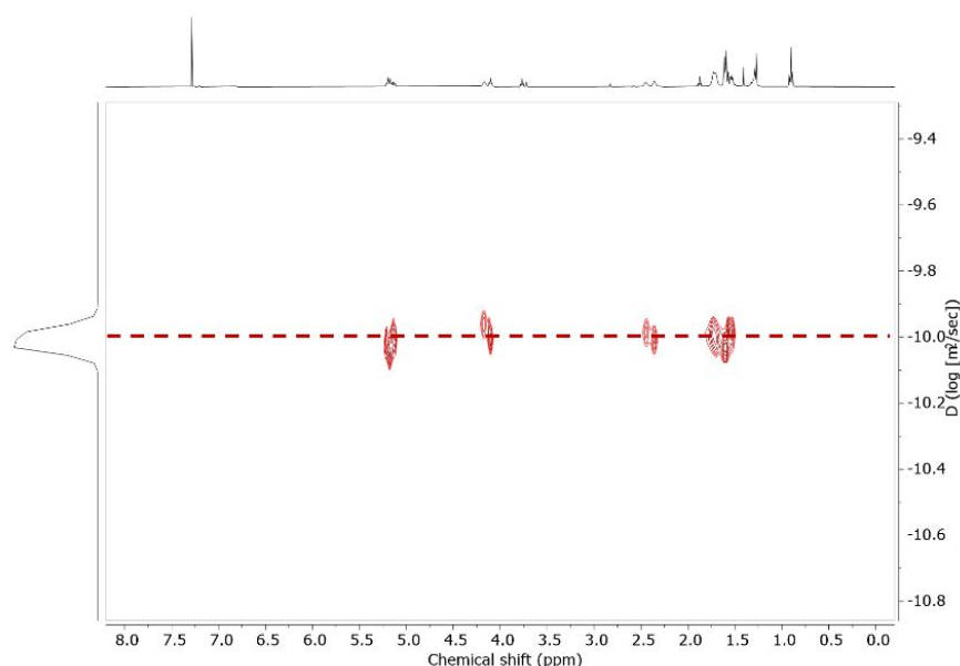
Figure 3: ^1\text{H} DOSY NMR spectrum of a poly(lactide-co- valerolactone) copolymer prepared using 3 . Reaction conditions: [\text{rac-LA}]_0 = [\delta\text{-VL}]_0 = 0.5\text{ M} in THF, [[\text{rac-LA}]_0/\mathbf{3}] = 10 , reaction time 20 min.
