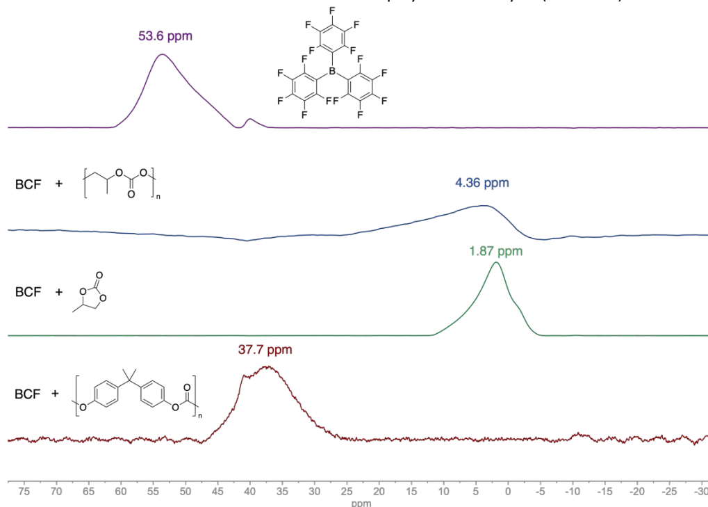
Figure 3. 11 B NMR spectra (160 MHz, CDCl 3 ) of BCF alone (top, purple) and in the presence of PPC (second, blue), PC (third, green), or PBPAC (bottom, red)
