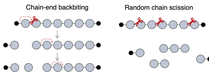
Figure 4. Schematic of two possible CDP pathways presented in this work. 31,50
