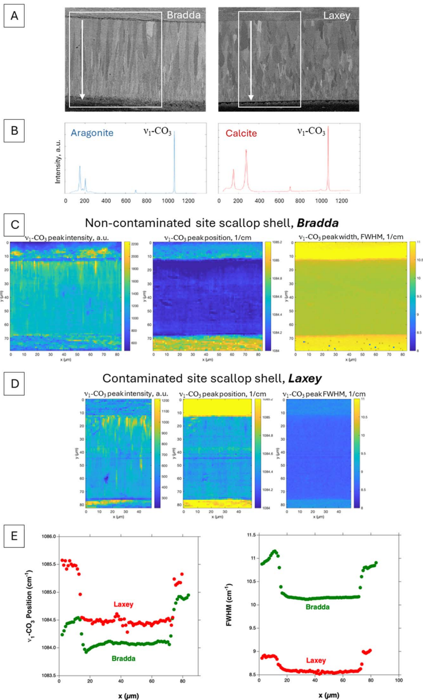
Fig. 8 (A) BSE images of a sample from non-contaminated (Bradda) and contaminated (Laxey) sites; (B) Raman spectra taken from the myostracum and foliated regions of the Bradda sample, (C) \nu_1\text{-CO}_3 Raman maps evaluating peak intensity, position and full width at half maximum of the Bradda and (D) and Laxey samples, (E) comparison of line profiles from top to bottom of the \nu_1\text{-CO}_3 Raman position and full width at half maximum for Bradda and Laxey samples.
