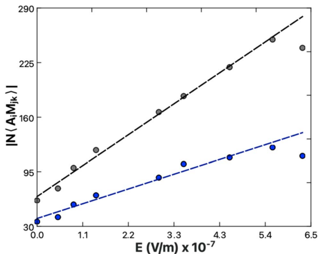
Fig. 7 3200 \text{cm}^{-1} (black) and 3400 \text{cm}^{-1} (blue) peak transition probabilities from spectral fits of Ca-exposed DPPS (Fig. 5B) plotted as a function of the electric field strength one Debye length away from the lipid surface (Table 1). The determined slopes, representing the relative \chi^{(3)} , are 3.4 \pm 0.1 \times 10^6 \text{ m V}^{-1} for the ice-like 3200 \text{cm}^{-1} and 1.6 \pm 0.1 \times 10^6 for the water-like 3400 \text{cm}^{-1} .
