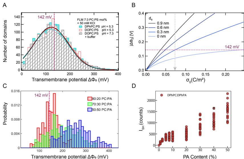
Fig. 5 Transmembrane potential distributions on FLMs and GUVs. FLMs: (A) transmembrane potential values per domain ( \langle\Delta\Phi_{\text{domain}}\rangle ), taken from 1 s SH images and averaged over 20 images) from 3 different symmetric FLMs composed of 70 : 30 mol% DPhPC : DPhPS (turquoise), 70 : 30 mol% DOPC : DOPS (red/white) immersed in a pH 5.3, 50 mM KCl solution, and the same DOPC : DOPS mixture but with 10 mM PBS buffer added to both sides (dashed grey). The lines are Gaussian fits to the data. (B) Computed values of the surface potential difference ( |\Delta\Phi_0| ) as a function of the surface charge density ( \sigma_0 ) plotted for different thicknesses of the Stern layer ( d_s ). The x axis spans a neutral surface up to a fully ionized DPhPS layer. (C) Transmembrane potential values per 20 \mu\text{m}^2 domains obtained for GUVs composed of DPhPC : DPhPA with 3 different mole% ratios of 1 : 1 (blue), 7 : 3 (green), and 8 : 2 (red). The solution inside the GUV contains 45 mM sucrose, and the solution outside the GUV contains 30 mM glucose and 5 mM \text{CaCl}_2 . (D) Bar graph showing how the distribution of average SH intensity per GUV changes for different GUVs prepared according to the same protocol. Each marker represents one GUV. Between 9 and 29 GUVs were imaged per lipid composition.
