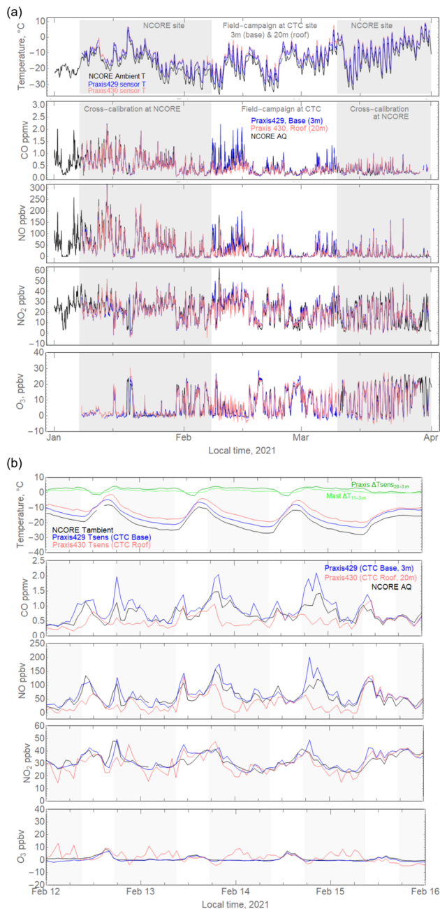
Fig. 1 (a) Time-series of hourly CO, NO, NO 2 , and O 3 gas abundances measured by low-cost electrochemical sensors in two instruments (Praxis 430, pink, and Praxis 429, blue) in downtown Fairbanks. Also shown are measurements by DEC air-quality monitors (black) at the Fairbanks NCORE EPA monitoring site. During January 9–February 7 and March 9–March 31, the sensors were co-located at NCORE (3 m), shaded regions, as part of cross-calibration. During February 7–March 9 the sensors were located at the CTC site (500 m south of NCORE) at the base (3 m height, Praxis 429, blue) and on the CTC building rooftop (20 m height, Praxis 430, pink), and show distinct differences in air composition.
