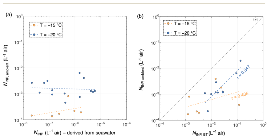
Fig. 11 Comparisons between ambient N_{\text{INP}} measured from impinger samples and coincident N_{\text{INP}} measured from (a) seawater and (b) BT-aerosol filters. The dashed lines indicate the linear regression in the logarithmic scale, and only the statistically significant ( p < 0.05 ) r values (correlation coefficients) are shown in the figure. The correlation coefficients of all data are given in Table A1.†
