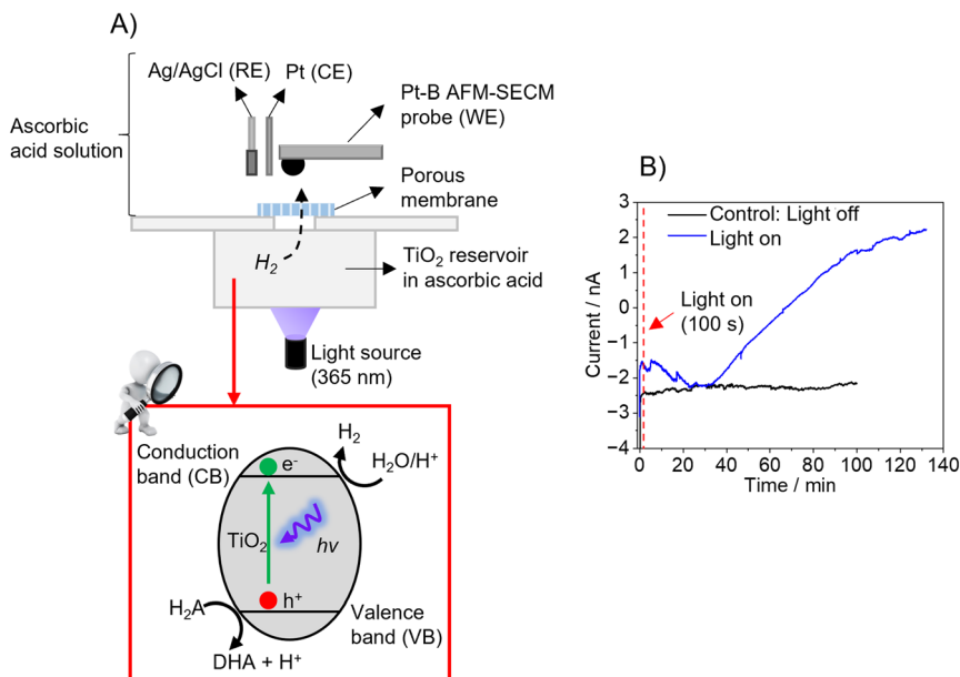
Fig. 3 (A) Schematic of the two-compartment setup used for the proof-of-principle \text{H}_2 measurement using the Pt-B AFM-SECM probe. (B) Chronoamperometry ( i-t curve) recorded at the Pt-B AFM-SECM probe ( E_{\text{probe}} = -0.05 V vs. Ag/AgCl) under illumination ( \lambda = 365 nm, blue line) and dark conditions (black line).
