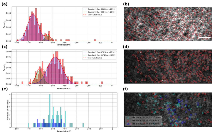
Fig. 4 Calculated onset potential probability histogram and corresponding fitted Gaussians for automatically detected scattering regions (a) on bare ITO coverslip, (c and e) on MoS 2 drop-cast ITO coverslip, using (c) high threshold (maximum number of detected features) or (e) low threshold, detection. Corresponding first frames of the recorded videos with selected regions for intensity analyses for (b) bare ITO coverslip (scale bar 5 \mu m), (d and f) MoS 2 drop-cast ITO coverslip. In (e and f) particles are classified into three categories: those detected in the first raw image and active during ORR (cyan), those active but not detected on the first image thresholding (blue) and detected on the first image and inactive (red). The distribution in (e) shows the onset potentials of detected and active particles (cyan) and not detected but active particles (blue).
