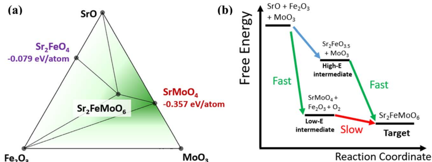
Fig. 5 (a) A ternary compound convex hull for the precursors used to synthesize \text{Sr}_2\text{FeMoO}_6 . (b) A reaction diagram for \text{Sr}_2\text{FeMoO}_6 , illustrating how the choice of a high-energy ternary oxide precursor will save more reaction energy for forming the target in the final step.
