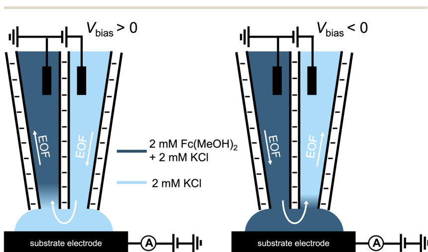
Scheme 2 Experimental setup for the \text{Fc}(\text{MeOH})_2 -KCl system utilized for Fig. 3–5. The left channel contains 2 mM \text{Fc}(\text{MeOH})_2 and 2 mM KCl (dark blue), while the right channel contains 2 mM KCl (light blue).
