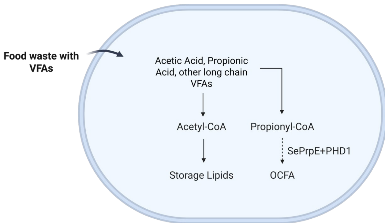
Figure 4. Volatile fatty acids metabolic pathways.
