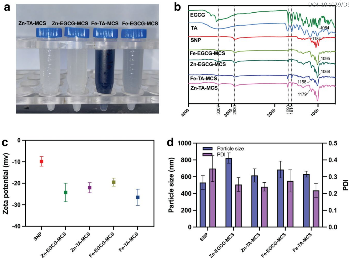
Figure 1. (a) Formulation of four metal-phenolic-network capped starch nanoparticles (MCS); (b) Fourier-transform infrared (FTIR) spectra; (c) zeta potential (pH=4); (d) Dynamic light-scattering analysis
