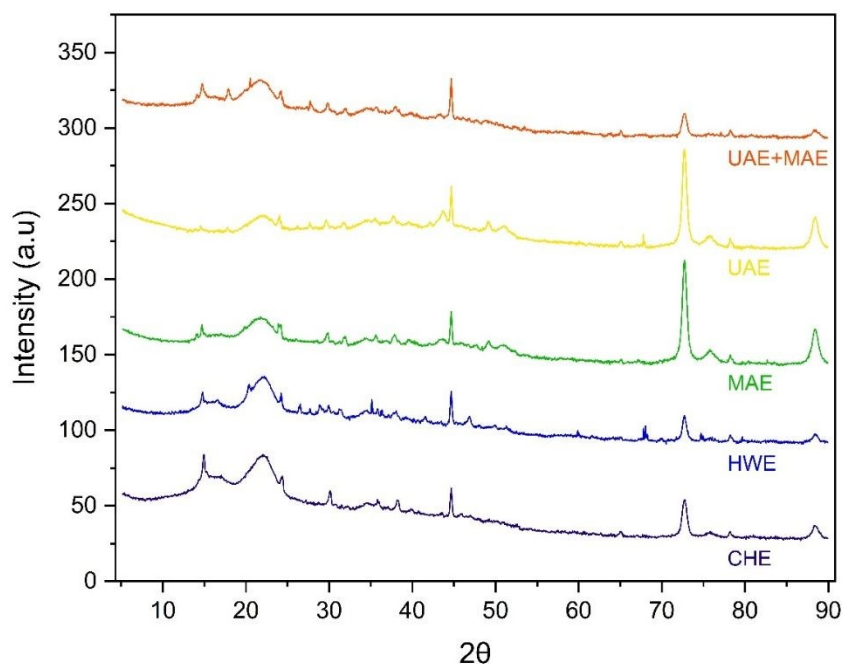
Fig.6 X-ray diffraction (XRD) patterns of dietary fibre obtained from banana pseudostem scutcher under different extraction treatments
